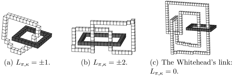
Fig. 2. Three different links between a 6-path \pi in black and a 18-path \kappa in white.
