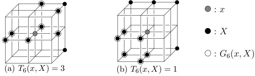
Fig. 1. Two examples of geodesic neighborhoods and topological numbers.
