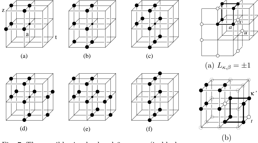
Fig. 7. The possible simple closed 6–curves (in black points) in N_{18}(x) up to rotations and symmetries.
