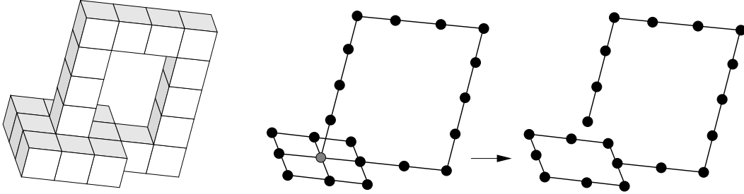
Fig. 4. When (n, \bar{n}) \in \{(6, 18), (6, 26)\} , the gray point can be removed without changing the number of tunnels in the object which is equal to 1 in both sets. However, this point is obviously not simple.
