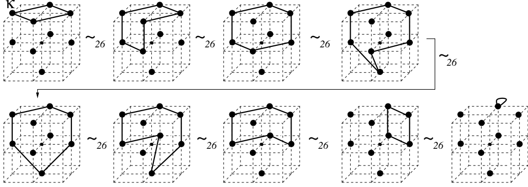
Fig. 10. A 26-homotopic deformation of the closed path \kappa .
