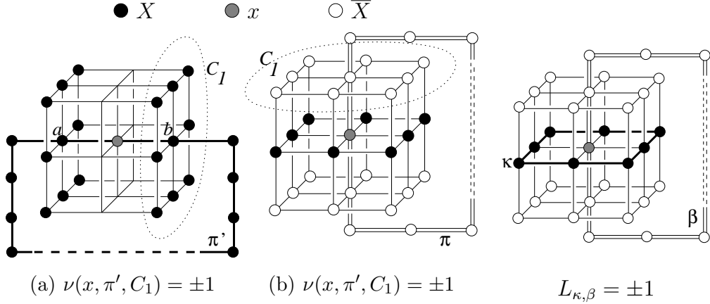
Fig. 5. Illustrations of the proofs of Propositions 14 and 19 Fig. 6. Idea of the proof of Proposition 18
