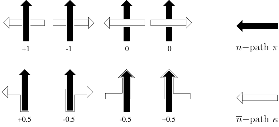
Fig. 3. Contributions associated with points where the two paths of a link overlap in a 2D projection of the link.
