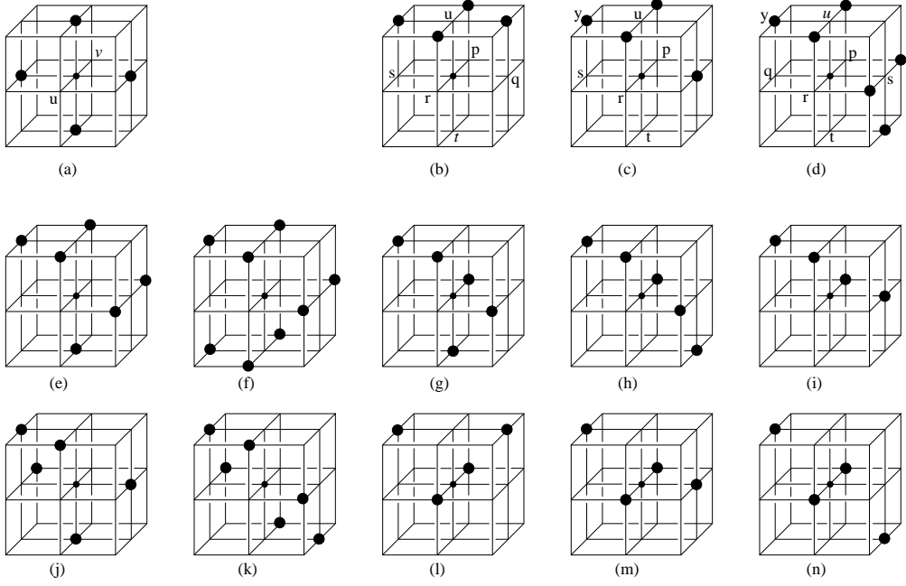
Fig. 9. The possible simple closed 26–curves in N_{26}(x) up to rotations and symmetries.
