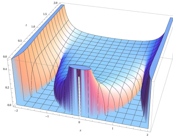
FIGURE 4. The density of \frac{\delta_{-1+\delta_1}}{2} *_t \frac{\delta_{-1+\delta_1}}{2} at the point x in function of x and t . The support fills progressively the interval [-2, 2] when t increases from 0 to 1, and then the distribution converges rapidly towards the arcsine distribution.
