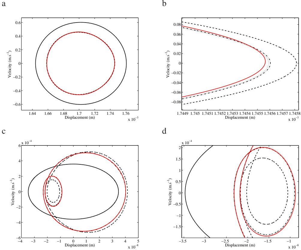
Figure 4: Limit cycles using the classical temporal integration and the modified HBM at \mu_0 ; — temporal integration, — 1 harmonic, - - 2 harmonics, - . - 3 harmonics, ... 10 harmonics; (b,d) zoom
