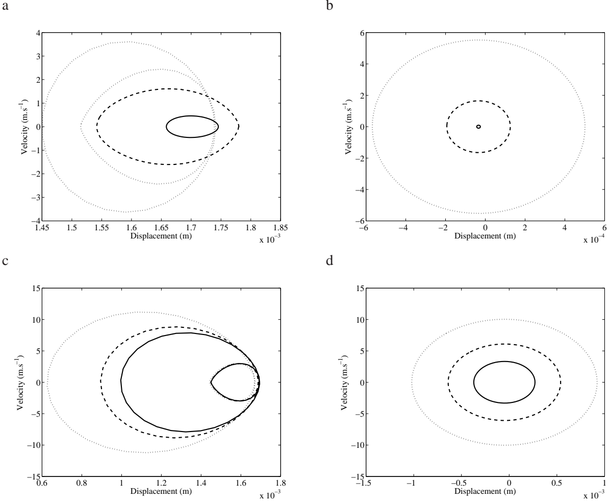
Figure 14: Limit cycles for non-equally damped modes and plotted for two different \mu (a-b) Limit cycles plotted at \mu = \mu_0 — 1 st case, - - 6 th case, ... 7 th case (c-d) Limit cycles plotted at \mu = 1.4\mu_0 ; — 1 st case, - - 6 th case, ... 7 th case; (a-c) Pad (b-d) Disc
