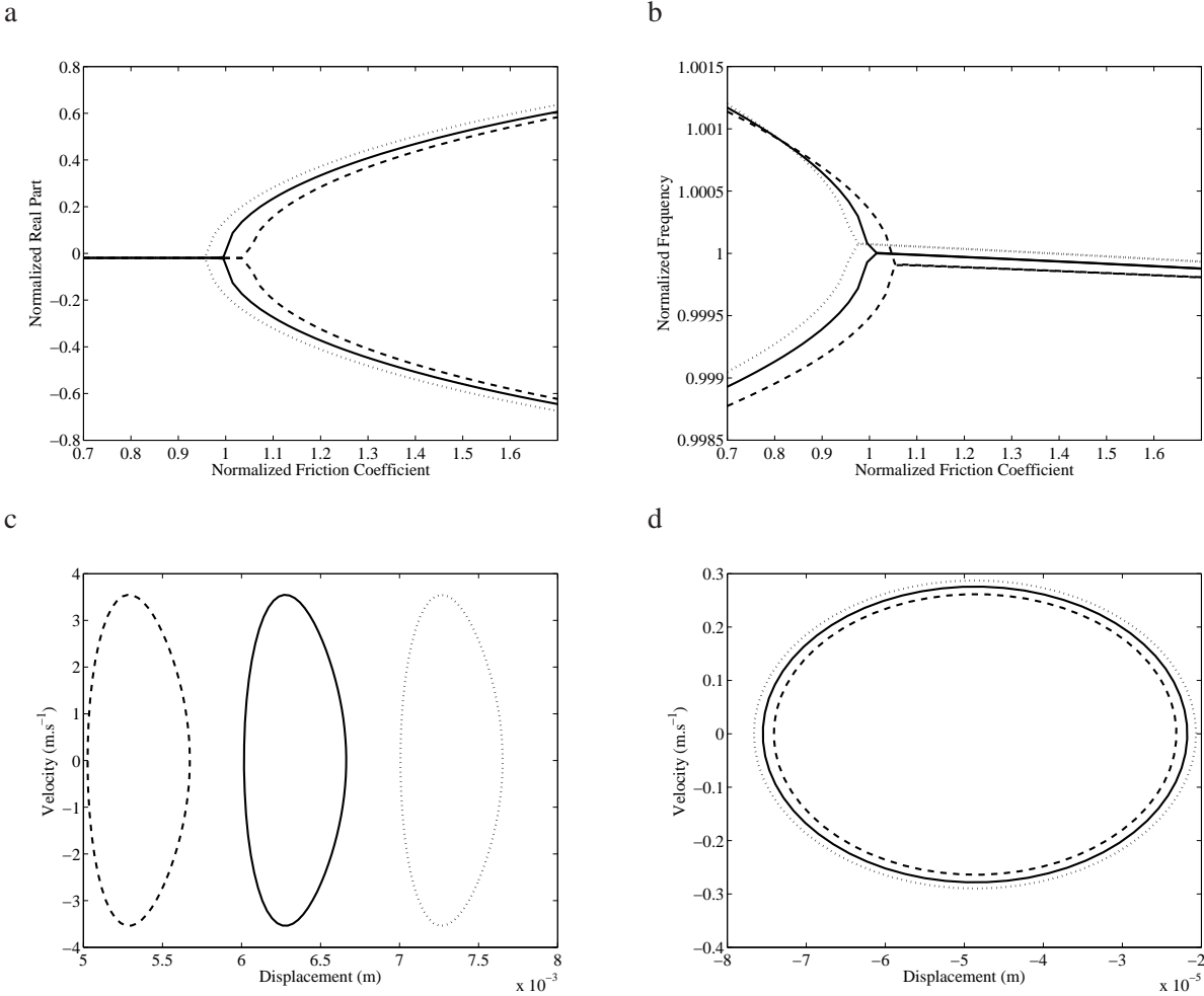
Figure 9: Influence of piston pressure; — P_0 , - - 0.8P_0 , ... 1.2P_0 (a) Evolution of real parts (b) Frequency coalescences; Limit cycles for (c) Pad, (d) Disc
