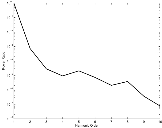
Figure 5: Power ratio for the first 10 harmonics
