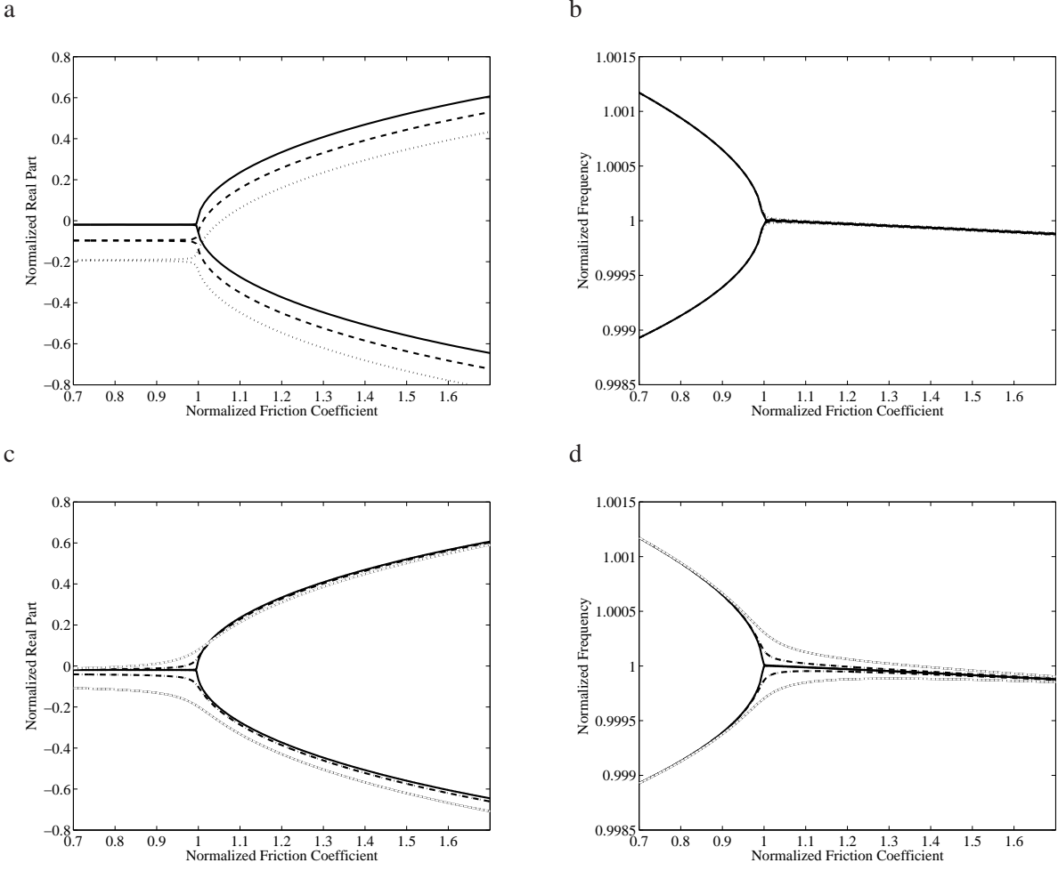
Figure 11: Evolution of real parts and frequency coalescences (a-b) equally damped: — 1 st case, - - 2 nd case, ... 3 rd case (c-d) non-equally damped: — 1 st case, - - 6 th case, ... 7 th case
