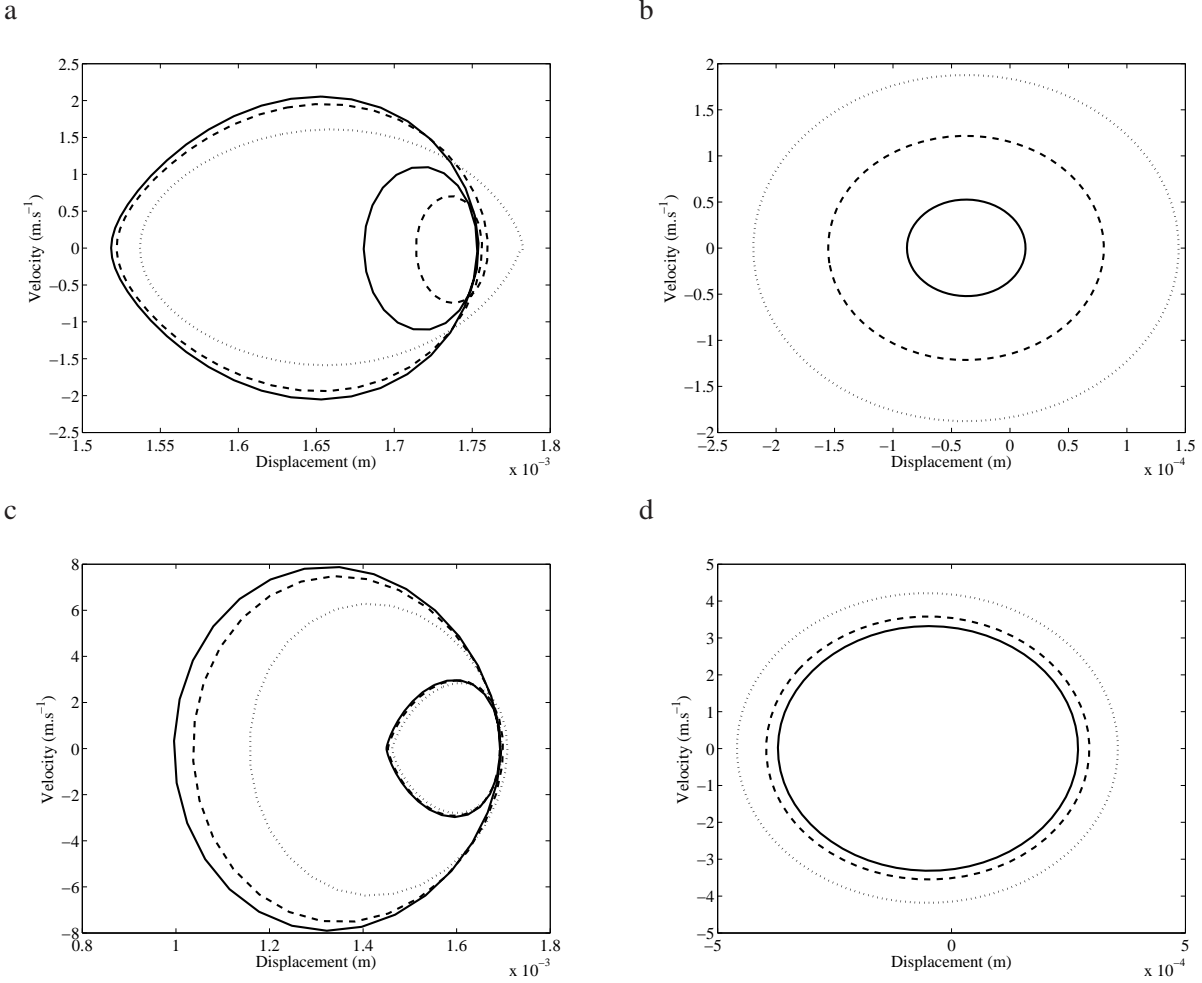
Figure 12: Limit cycles for equally damped modes and plotted for two different \mu (a-b) Limit cycles plotted at \mu = 1.07\mu_0 — 1 st case, - - 2 nd case, ... 3 rd case (c-d) Limit cycles plotted at \mu = 1.4\mu_0 — 1 st case, - - 2 nd case, ... 3 rd case; (a-c) Pad, (b-d) Disc
