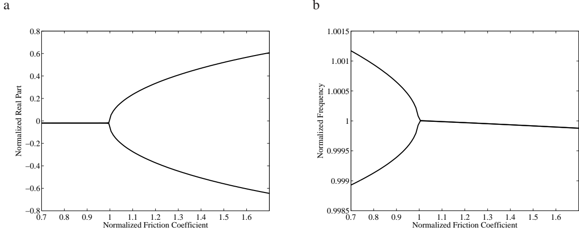
Figure 2: Stability analysis (a) Evolution of the real parts of the stable and unstable modes (b) Coalescence of the two corresponding eigenvalues
