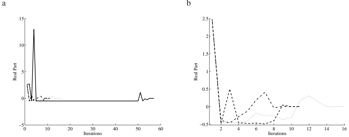
Figure 6: Evolution of the real part; — 1 harmonic, - - 2 harmonics, -.- 3 harmonics, ... 10 harmonics (a) all cases (b) zoom on 2, 3 and 10 harmonics
