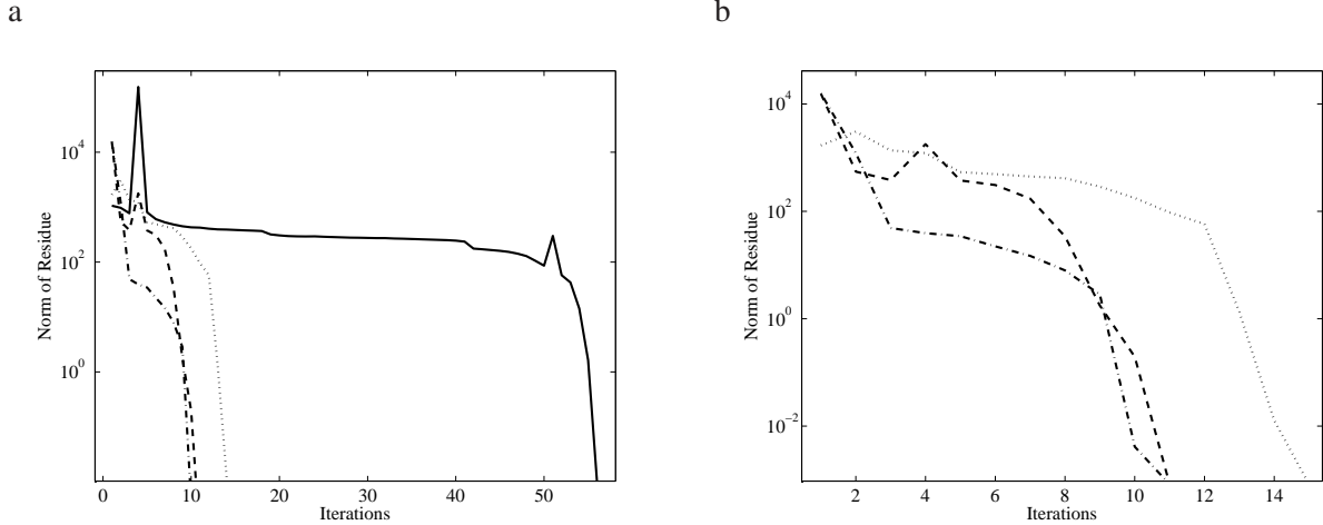
Figure 7: Evolution of residues during optimization; — 1 harmonic, - - 2 harmonics, -.- 3 harmonics, ... 10 harmonics (a) all cases (b) zoom on 2, 3 and 10 harmonics
