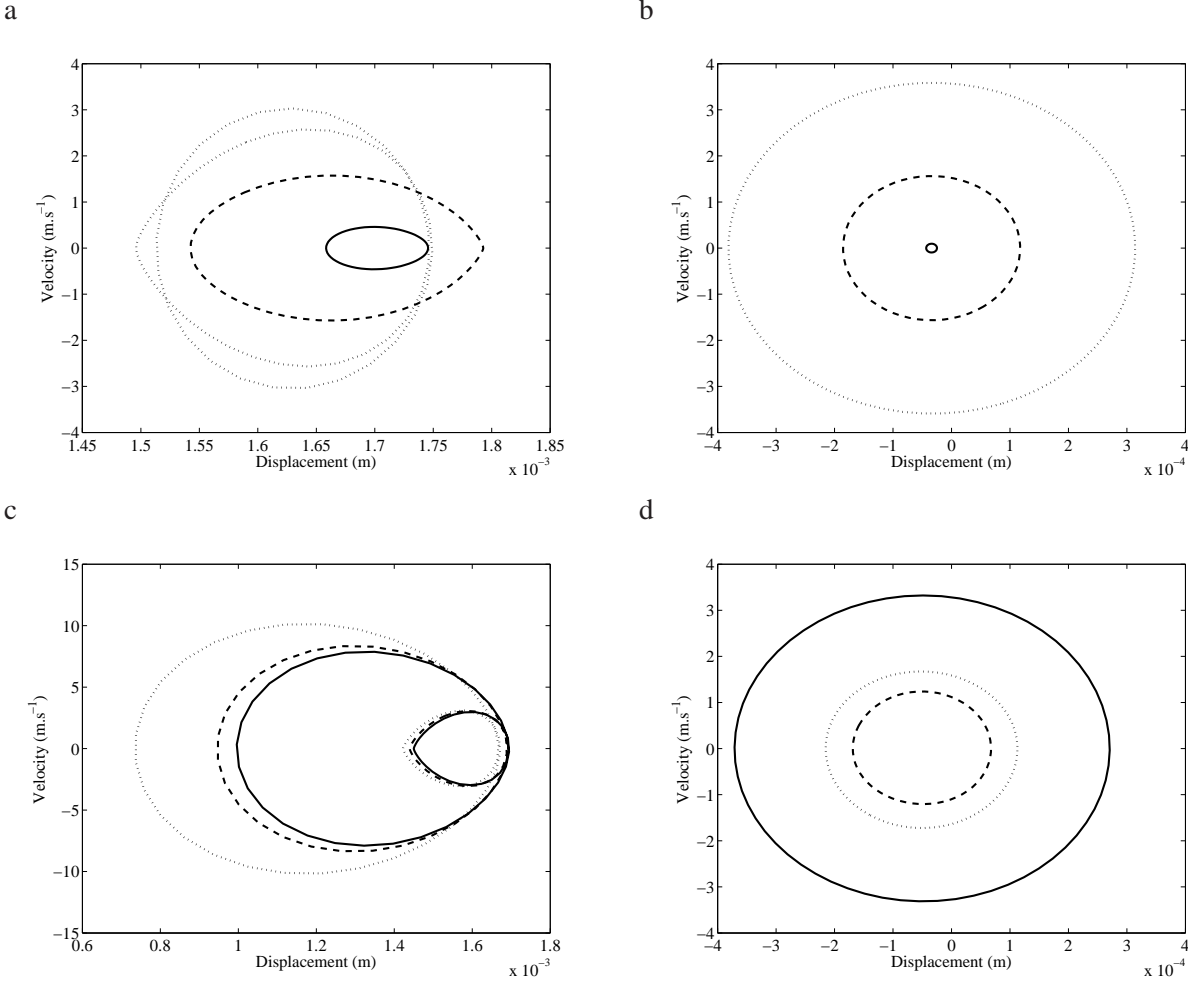
Figure 13: Limit cycles for non-equally damped modes and plotted for two different \mu (a-b) Limit cycles plotted at \mu = \mu_0 — 1 st case, - - 4 th case, ... 5 th case (c-d) Limit cycles plotted at \mu = 1.4\mu_0 — 1 st case, - - 4 th case, ... 5 th case; (a-c) Pad, (b-d) Disc
