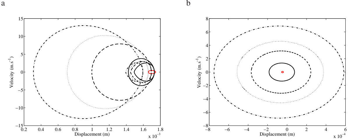
Figure 8: Limit cycles for pad and disc nodes; — \mu_0 , — 1.2\mu_0 , - - 1.4\mu_0 , ... 1.6\mu_0 , -.-. 2\mu_0 (a) Pad, (b) Disc
