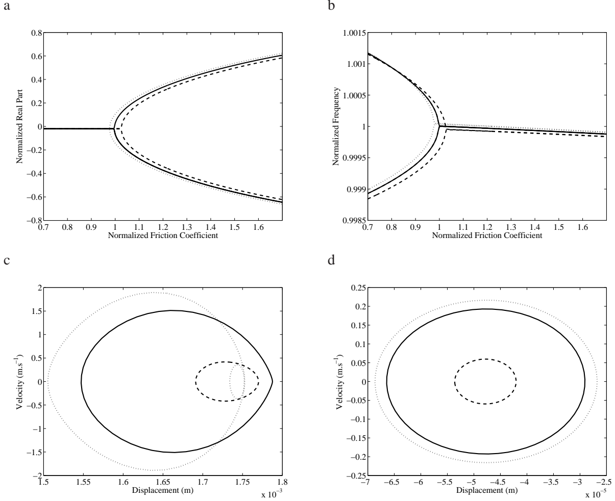
Figure 10: Influence of contact stiffness; — k_s , - - 0.7k_s , ... 1.3k_s (a) Evolution of real parts (b) Frequency coalescences; Limit cycles for (c) Pad, (d) Disc
