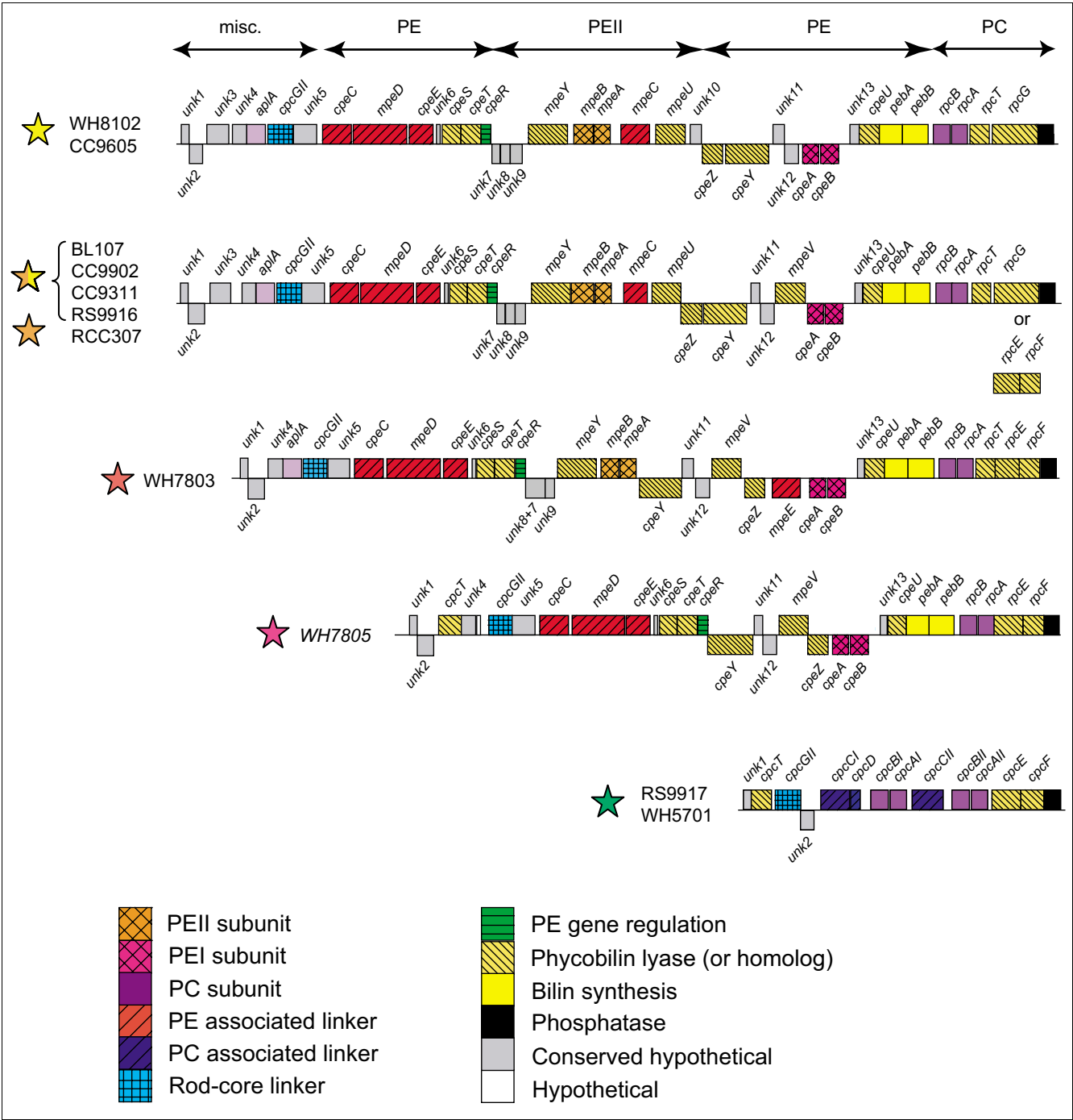
Figure 4 Comparison of PBS rod gene regions of the different pigment types of marine Synechococcus . Rectangles above and below the lines have a length proportional to the size of ORFs and correspond to the forward and the reverse strand, respectively. In several genomes, the sense of the rod region was inverted so that the regions all appear in the same direction. For the group formed by the chromatic adapters and RCC307, a few variations can be found with regard to the region shown here, which corresponds to BL107. First, the lyase-encoding gene(s) located near the 3'-end can either be a rpcE-F operon or rpcG , a pecEF -like fusion gene (see text). Second, the gene organization at the 5'-end can vary: unk1 is located elsewhere in the genome of RCC307 and the gene following unk2 is either the lyase gene cpcT in RS9916 and RCC307, unk3 in BL107 and CC9902, or none of these in CC9311. Colored stars indicate the pigment type of each strain (see Figure 1 for color code).
