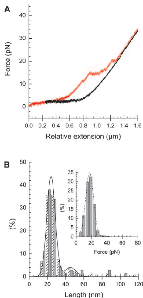
FIG. 2. Stretching profile of the reconstituted 5 S nucleosomal arrays. A , force/extension curve of the stretching cycle (extension in red, relaxation in black). B , the distribution of disruption lengths in 1 \times TE, 100 mM NaCl buffer in the absence (shaded bars) and in the presence (gray bars) of 1 mM MgCl_2 . Inset, the distribution of the threshold forces (without MgCl_2 ).
