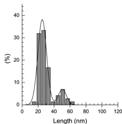
FIG. 7. Distribution of disruption lengths of reconstituted 5 S nucleosomal arrays in presence of nucleosomes at a concentration of 100 \mu\text{g}/\text{ml} . Note the significant increase in the population of disruption with length around 50 nm.
