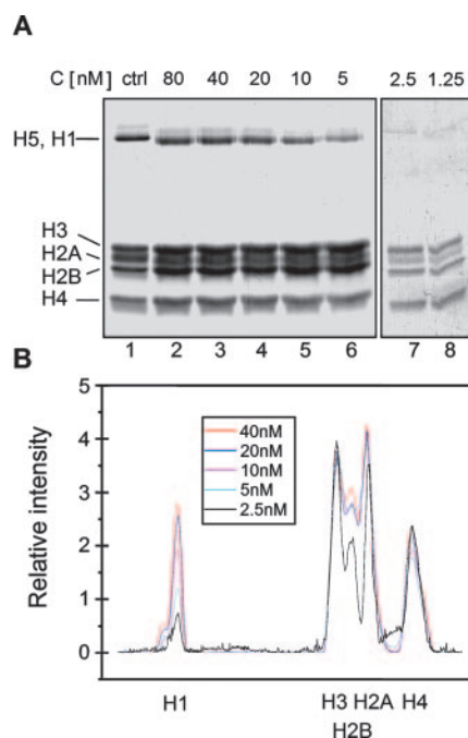
FIG. 6. Stepwise release of histones at very low chromatin concentrations. A , chromatin aliquots. 4 \mu\text{g} (lanes 2–6) and 2 \mu\text{g} (lanes 7 and 8) were diluted in 1\times PBS buffer to the indicated concentrations. Positions of the linker histones (H1 and H5) as well as those of the core histones are designated. B , scans of the samples shown in A . Since the amount of loaded material on lanes 7 and 8 was 2-fold smaller, a normalization of the intensity of the H3 band relative to histone H3 at 20 nM (lane 3) was applied. Note that upon lowering the chromatin concentration, the first histones released from chromatin are the linker histones followed by the H2A-H2B dimers.
