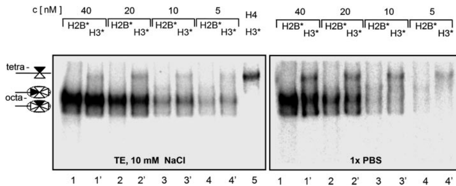
FIG. 5. Electrophoretic mobility shift assay of reconstituted nucleosomes at very low concentrations under different conditions. The nucleosomes contained either ^{32}\text{P} -labeled H3 ( \text{H3}^* nucleosomes) or ^{32}\text{P} -labeled H2B ( \text{H2B}^* nucleosomes). The tetrameric particles contained ^{32}\text{P} -labeled H3 ( \text{H3}^* -H4 particles). On the left, positions of the intact nucleosomes ( octa ; labeled H2B and H3, respectively) and of the tetrameric particles ( tetra ) are shown. At higher ionic strength ( 1\times PBS), the H2A-H2B dimer is completely released from the octamer when only partial release of the H2A-H2B dimer is observed at low ionic strength ( 1\times TE, 10 mM NaCl).
