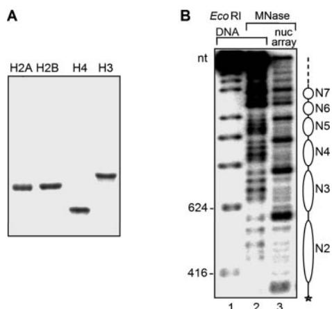
FIG. 1. A , 18% SDS-PAGE analysis of recombinant histones used for reconstitution; B , micrococcal nuclease digestion pattern of naked 5 S rDNA arrays (lane 2) and reconstituted nucleosomal 5 S rDNA arrays (lane 3). The positions of the nucleosomes are designated on the right. Lane 1, molecular mass marker. nt , nucleotides.
