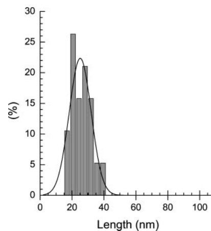
FIG. 4. Distribution of disruption lengths of histone H3-H4 tetramers reconstituted on the 5 S DNA arrays. The stretching was carried out at 1\times TE, 100 mM NaCl buffer. Contrary to the nucleosome arrays reconstituted with histone octamer or to native chromatin (Figs. 2 and 3), the distribution of lengths entirely misses the longer disruptions.
