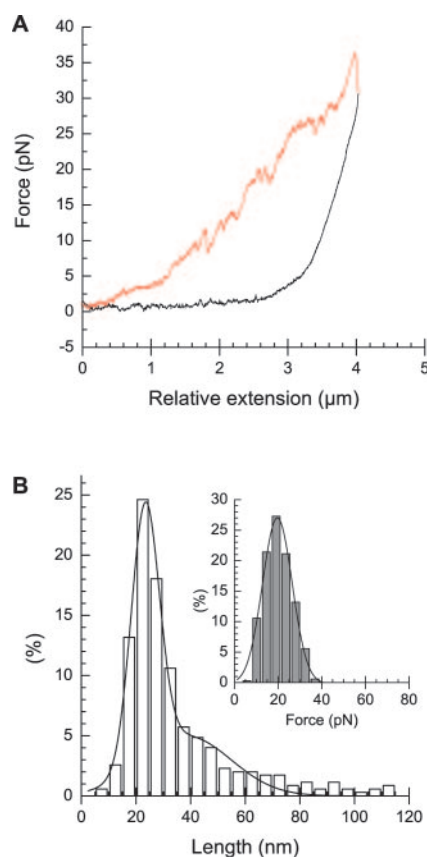
FIG. 3. Stretching profile of the chromatin isolated from the chicken erythrocyte nucleus in 1\times TE, 100 mM NaCl buffer. A, an example of the force/extension curve; B, the distribution of disruption lengths. Inset, the distribution of the threshold forces. Note the higher proportion of disruption lengths around \sim 40 nm compared with that of reconstituted nucleosomal arrays.
