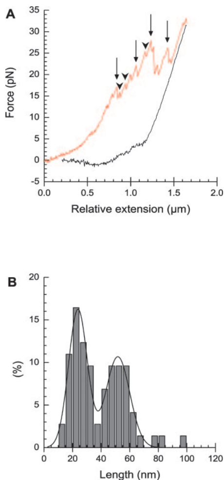
FIG. 8. Stretching profile of the chicken erythrocyte chromatin under optimized conditions (see “Materials and Methods”). A, force/extension curve (stretching in red, relaxation in black); the arrows mark the long \sim 50 -nm disruptions, and the arrowheads mark the short \sim 25 -nm ones. B, the distribution of disruption lengths. The second well separated maximum at \sim 50 nm approaches similar statistical weight as the one at \sim 25 nm.
