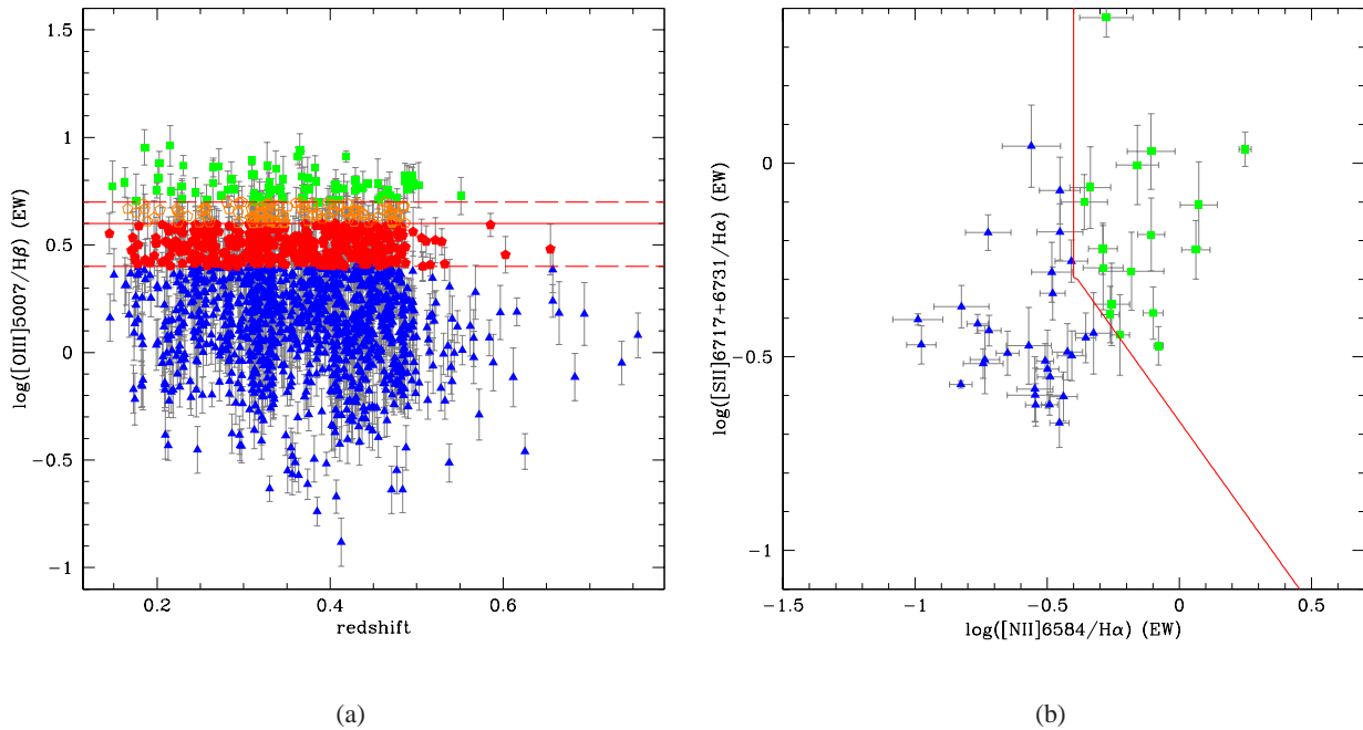
Figure 5. Intermediate spectral classifications of 1479 (a) and 43 (b) narrow emission-line galaxies. The two plots show the intermediate diagnostic diagrams, used in the redshift bins 0.4 < z < 0.5 (a) and 0.0 < z < 0.2 (b), or in other redshifts bins for galaxies with insufficient number of detected emission lines (therefore not classified with the red or blue diagnostic). The emission-line ratios – i.e. [\text{OIII}]\lambda 5007/\text{H}\beta , [\text{SII}]\lambda\lambda 6717+6731/\text{H}\alpha , and [\text{NII}]\lambda 6584/\text{H}\alpha – are calculated using equivalent widths. The red solid lines are the empirical separations defined by Lamareille (2006). In the left panel, the dashed lines delimit the error domain where both star-forming and AGNs galaxies show similar blue line ratios. The star-forming galaxies are plotted as blue triangles, the Seyfert 2 galaxies as green solid squares, the candidate star-forming galaxies as red solid pentagons, and the candidate AGNs as orange open pentagons. The error bars are shown in grey.
