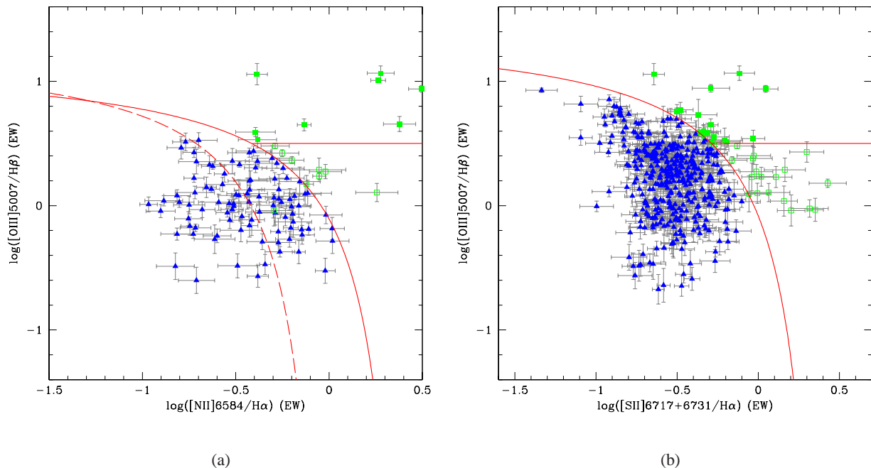
Figure 3. Red spectral classification of 412 narrow emission-line galaxies in the redshift bin 0.2 < z < 0.4 . The emission-line ratios – i.e. [\text{OIII}]\lambda 5007/\text{H}\beta and [\text{NII}]\lambda 6584/\text{H}\alpha (a) or [\text{OIII}]\lambda 5007/\text{H}\beta and [\text{SII}]\lambda \lambda 6717+6731/\text{H}\alpha (b) – are calculated using equivalent widths. The red solid curves are the semi-empirical separations defined by Kewley et al. (2001). The dashed line is the separation proposed by Kauffmann et al. (2003a). The star-forming galaxies are plotted as blue triangles, the Seyfert 2 galaxies as green solid squares, the LINERs as green open squares. The error bars are shown in grey.
