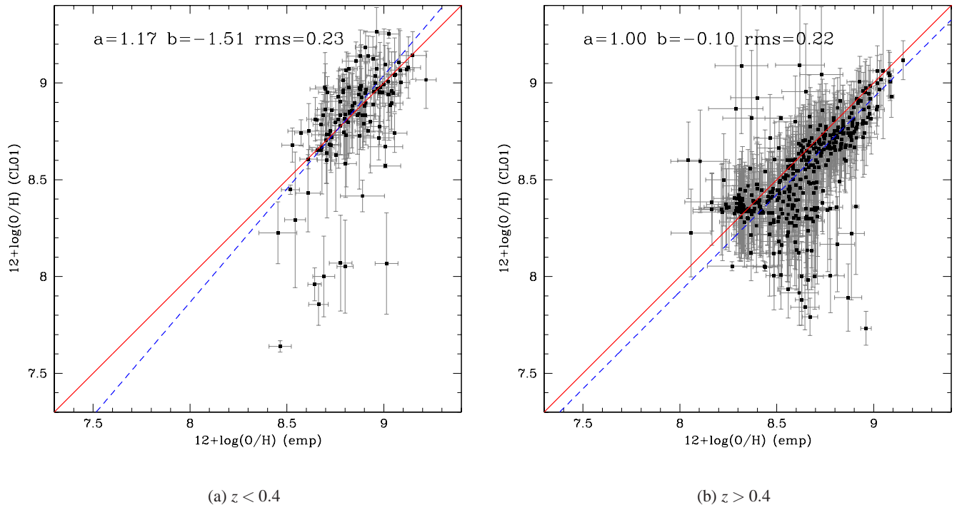
Figure 10. Comparison between empirically-calibrated ( x -axis), and CL01 metallicities ( y -axis) for our whole sample of star-forming galaxies. The red solid line shows the y = x relation, while the blue dashed line is a least-square fit to the data points. The parameters of the fit are given in the two plots ( a : slope, b : zero-point).
