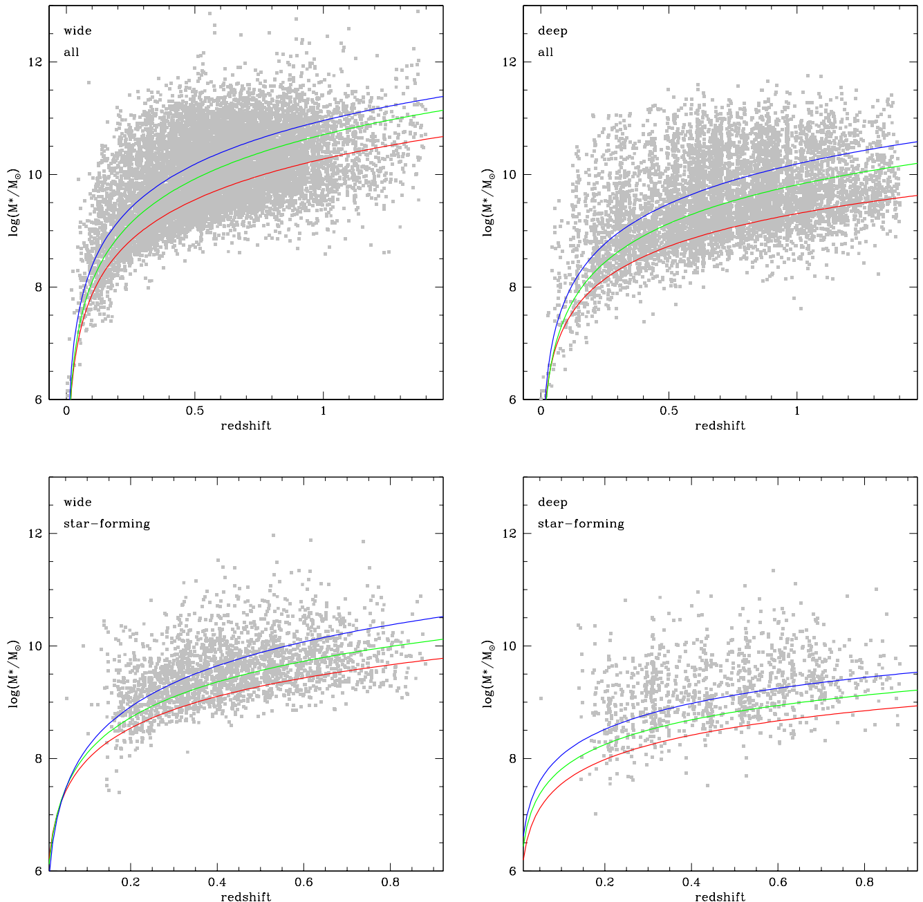
Figure 8. Stellar mass estimates (in logarithm of solar masses), as a function of redshift, of the galaxies in our samples: left: the wide sample, right: the deep sample, top: all galaxies (except broad-line AGNs), bottom: only star-forming galaxies (see Sect. 2.2). The red, green and blue curves illustrate respectively the 50%, 80% and 95% mass-to-light completeness levels (see text for details).
