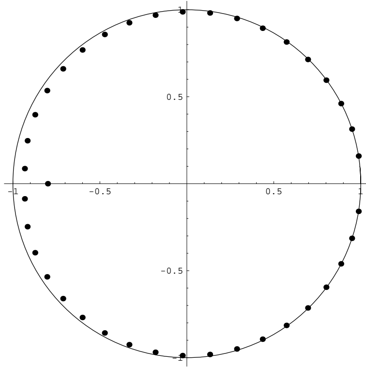
Figure 6. Galois conjugates ( \neq \beta ) of the Perron number \beta = 9.999\dots , dominant root of P_\beta(X) = X^{40} - 9\sum_{i=1}^{39} X^i - 4 , and confluent Parry number ( \beta is a Pisot number). The absence of beta-conjugates is controlled by the great regularity of the angular distribution of the Galois conjugates, by Theorem 4.1.
