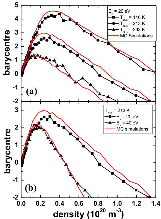
FIG. 8: (Color on line) Evolution of the size distribution barycentre as a function of the density of sodium atoms in the cell for \text{Na}_{90}^+ for (a) three different initial temperatures (the kinetic energy is E_k = 20 \text{ eV} ) and (b) two different kinetic energies ( T = 213 \text{ K} ). Full lines are the results of Monte Carlo simulations (see Section VI).
