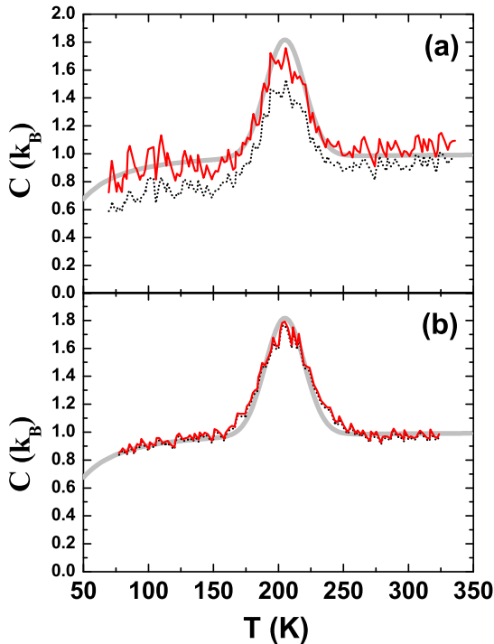
FIG. 10: (Color online) The thick solid line is the caloric curve introduced in the simulation ( L = 8 meV/atom, T_f=205 K and \Delta T= 30 K). The dotted curves correspond to the caloric curves obtained by setting the second derivative in Eq. 21 to 0 whereas for the curves in thin solid line it is taken into account. The top panel correspond to \bar{\tau} = 5.3 and the bottom one to \bar{\tau} = 10.6
