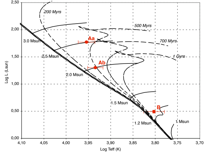
Fig. 9. Positions of \delta Vel Aa, Ab and B in the HR diagram, with the isochrones and isomass curves from Girardi et al. (2000) overplotted.
