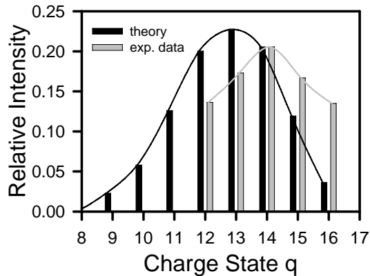
Figure 4: Comparison of experimental and theoretical charge state distributions obtained at 6 \times 10^{16} W/cm 2 . The experimental distribution was obtained from spectrum 3b) assuming mean fluorescence yields \langle \omega_{12+} \rangle = 0.19 , \langle \omega_{13+} \rangle = 0.24 , \langle \omega_{14+} \rangle = 0.31 , \langle \omega_{15+} \rangle = 0.49 , \langle \omega_{16+} \rangle = 0.45 . Experimental data on charge states q < 12+ could not be extracted. Full lines to guide the eye.
