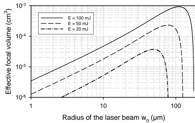
Figure 2: Dependence of the time - averaged effective focal volume on the beam waist for different laser energies. For an intensity threshold and pulse duration of 1.4 \times 10^{15} W/cm 2 and 60 fs respectively, each V_{eff.foc} displays a pronounced maximum.
