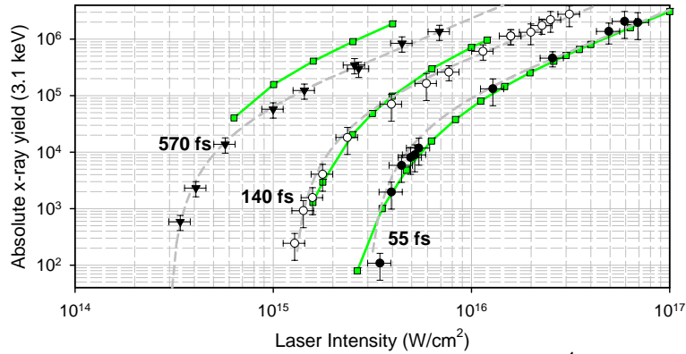
Figure 8: X-ray yield from argon clusters with \langle N \rangle \sim 3.7 \times 10^4 atoms as a function of laser peak intensity at 800 nm for different pulse durations of \tau=55 , 140 and 570 fs. Gray dashed lines correspond to the fitted effective focal volume and full lines with squares to the simulation data.
