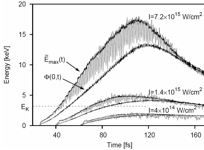
Figure 7: Time evolution of the maximum electron kinetic energy (gray) in the high density core of the cluster for three peak laser intensities, I=7.2 \times 10^{15} W/cm 2 (upper curve), I=1.4 \times 10^{15} W/cm 2 (center curve) and I=4 \times 10^{14} W/cm 2 (lower curve) and pulse duration \tau = 60 fs. The dashed horizontal line marks the neutral argon K-shell binding energy E_K=3.2 keV. Each curve is delimited below by the electrostatic potential \Phi(r=0,t) at the center of the cluster and above by \tilde{E}_{\max}(t) = \Phi(r = 0,t) + F_{\text{osc}}^2 / (2\omega^2) (see text).
