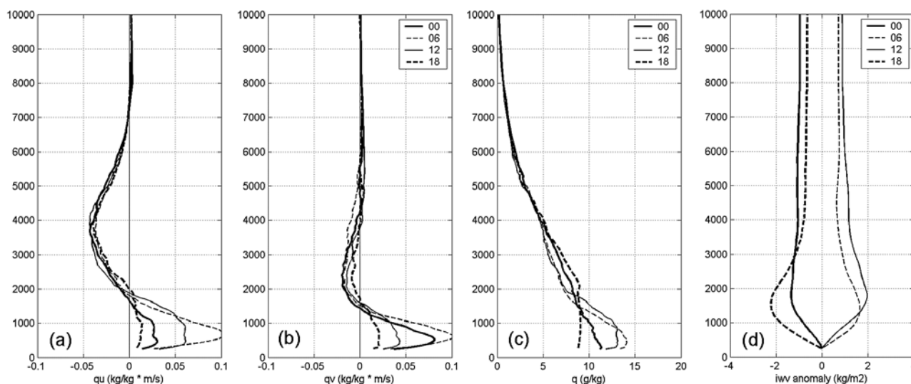
Figure 12. Radiosonde profiles averaged over the month of May 2006 at Niamey: (a) zonal and (b) meridional moisture flux, (c) specific humidity, and (d) PWV integrated from the surface to level z . The humidity profiles have been adjusted to fit the total PWV values measured by GPS.
