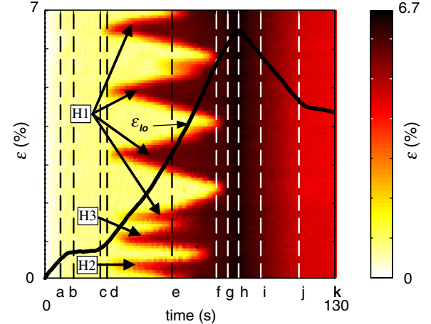
Fig. 7. Coloured map showing the time evolution of \epsilon(P) at the spatial points P located on the vertical dashed line plotted in Fig. 3(c). Superimposed curve: time evolution of the average axial strain \epsilon_{i0} .
