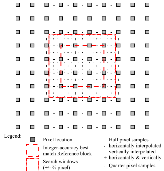
Figure 3. Sub-pixel search window and necessary data to compute quarter-pixel samples for a 4 \times 4 block
