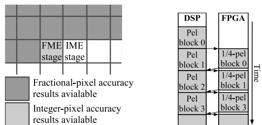
Figure 10. Block-level pipeline implementation
