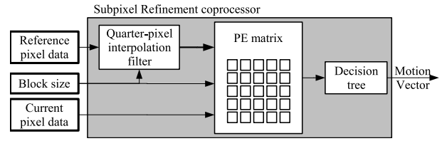
Figure 4. Overall VLSI architecture
