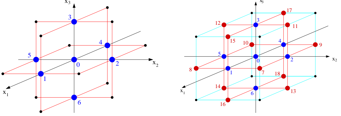
Figure 22: Stencils for D3Q7 and D3Q19 lattice Boltzmann schemes
