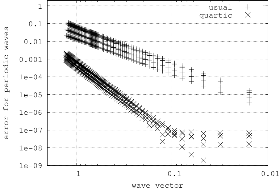
Figure 1: Precision of D2Q5 scheme for thermic test case, “one point” simulation. Different curves correspond to different orientation of the wave-vector with respect to the axis, showing the angular dependence of the next order.
