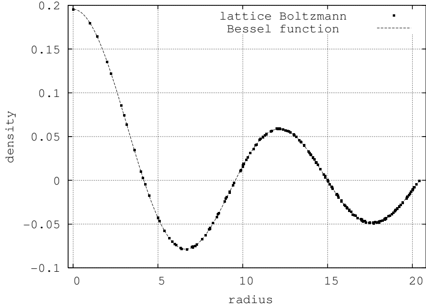
Figure 4: D2Q5 scheme for thermics inside a circle. Eigenmode n = 4 , \ell = 0 . Quartic parameters for lattice Boltzmann scheme.
