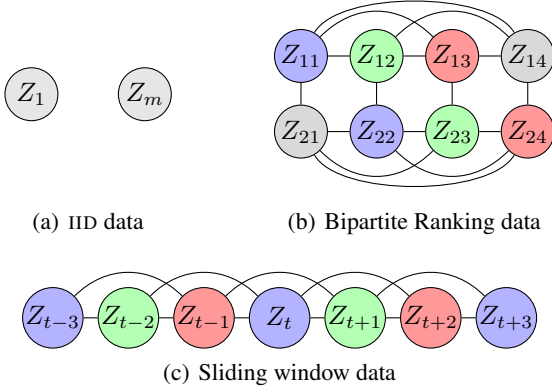
Figure 1: Dependency graphs for the different settings described in section 4: (a) when the data are IID, the dependency graph is disconnected and the fractional number is \chi^* = 1 ; (b) a dependency graph obtained for bipartite ranking from a sample containing 4 positive instances and 2 negative instances; nodes of the same color are independent and \chi^* = 4 ; (c) a dependency graph obtained with the technique of sliding windows for sequence data, for a window parameter r = 1 (see text for details): \chi^* = 2r + 1 .
