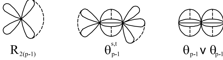
Figure 2: The graphs which determine H^*(Out(F_{2p-2}); \mathbb{F}_p) for p > 3 and * > 2p - 3 .
