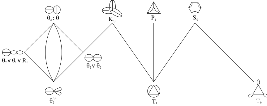
Figure 4: The K_{3,3} component of Out(F_4) \setminus (K_4)_s
