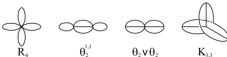
Figure 1: The graphs whose automorphism groups determine H^*(\text{Out}(F_4); \mathbb{F}_3) for * > 5 .
