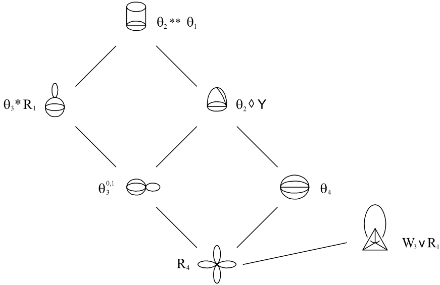
Figure 3: The rose component of Out(F_4) \setminus (K_4)_3 .
