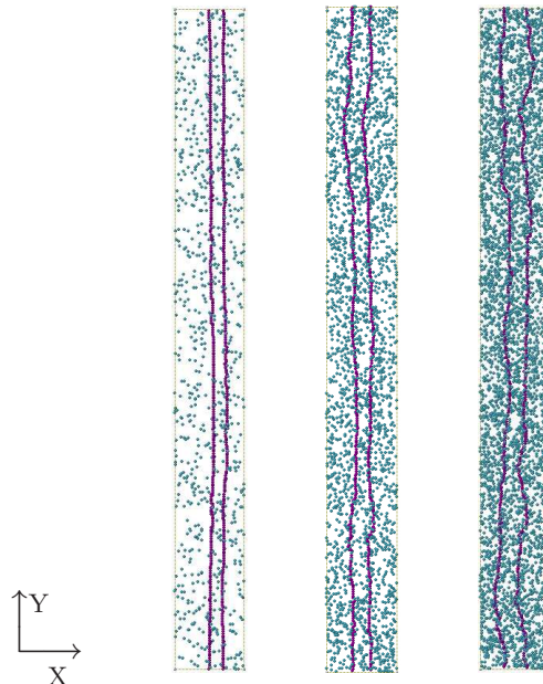
FIG. 1: (color online) View of the (1\bar{1}1) glide plane and the dissociated screw dislocation in the Ni(Al) simulated solution at various concentrations: C_{Al} = 2 at. % (lhs), C_{Al} = 6 at. % (center) and C_{Al} = 10 at. % (rhs). The box size is 300 b along Y, 32 b along X and 34 b along Z (orthogonal to this paper sheet). The Shockley partials are colored in violet and the Al atoms in blue. The external shear stress has been fixed to one half of the CRSS.
