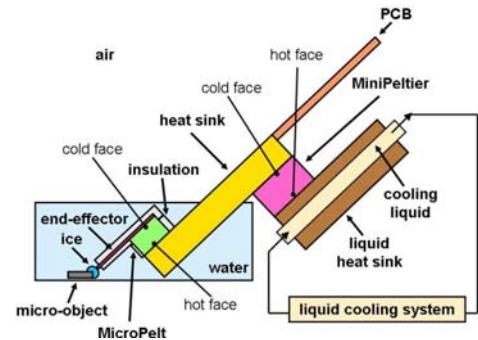
Fig. 2. Submerged Freeze System Principle.
