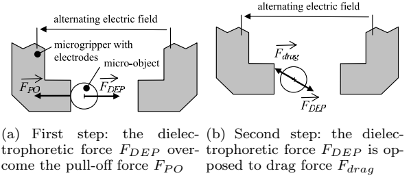
Fig. 2. Principle of the dielectrophoretic release
