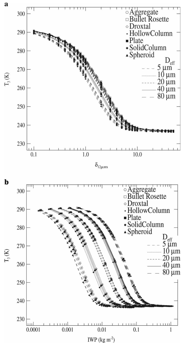
FIG. 3. Dependence of the brightness temperature T_3 at 12\ \mu\text{m} on (a) the optical depth \delta_{12\mu\text{m}} at 12\ \mu\text{m} and (b) IWP for all cloud microphysical models. All particle shapes and effective sizes are considered in calculations, assuming individual ice particles under the same conditions as in Fig. 2.
