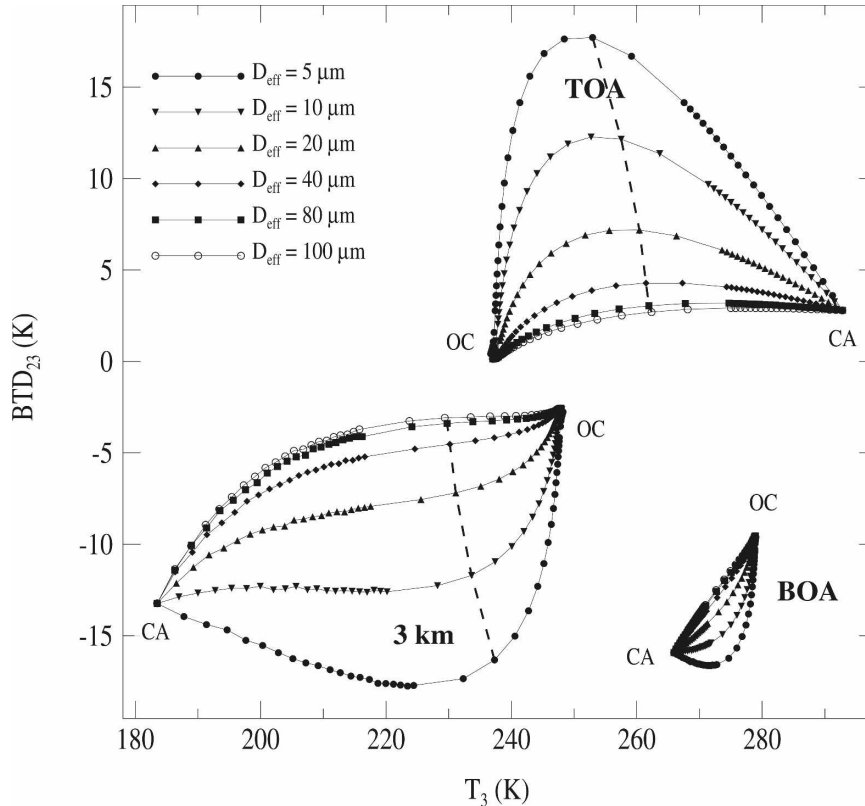
FIG. 2. BTD_{23} as a function of T_3 for a cirrus cloud with various effective sizes D_{\text{eff}} , assuming individual ice particles with an aggregate shape. The three sets of arches correspond to simulations performed at the TOA, BOA, and at 3-km altitude (3 km). The cloud is located between 9 and 10 km (237–243 K) for the standard tropical atmosphere from McClatchey et al. (1972). In the arches, CA and OC symbols refer to clear atmosphere and opaque cloud situations, respectively. The vertical dashed lines correspond to an optical depth equal to 2.
