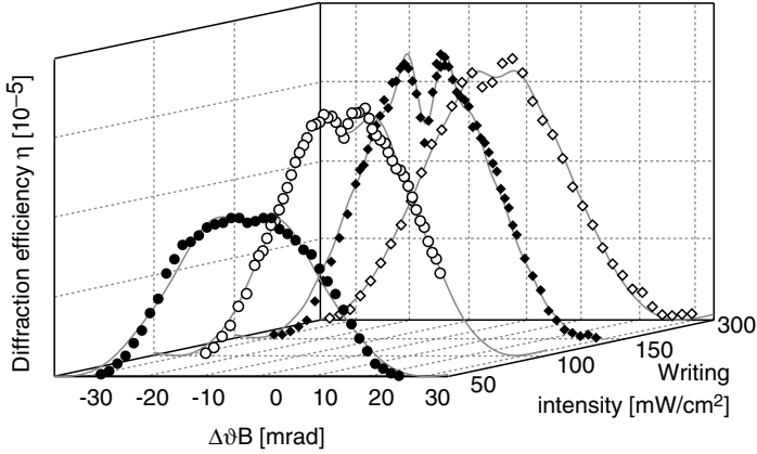
FIGURE 7.4. Measured internal angular selectivity of the diffraction efficiency for isotropic Bragg diffraction obtained in a 47\mu\text{m} thin sample of \text{KNbO}_3 for different ultraviolet writing intensities ( \lambda = 364\text{ nm} , grating spacing \Lambda = 0.5\mu\text{m} , grating vector along the c axis). The modulation depth is m = 0.2 and all the light beams are p -polarised. The solid lines are calculated from a simple model involving two grating components. See [15] for details.
