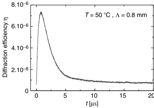
FIGURE 7.8. Dynamics of the diffraction efficiency in \text{Sn}_2\text{P}_2\text{S}_6 under pulsed grating recording at 532\text{ nm} . Pulse length = 50\text{ ns} ; Fluence = 100\text{ }\mu\text{J/cm}^2 . (After [45])
