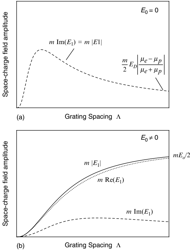
FIGURE 7.2. Dependence of space-charge field amplitude on grating spacing for interband photorefractive effects in absence of deep traps (4). a) No applied field; b) With externally applied field.
