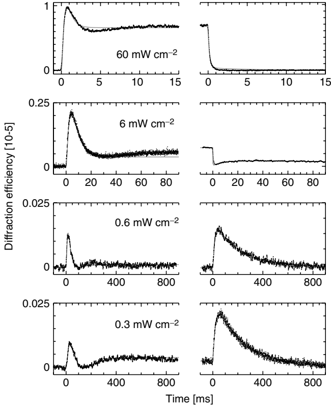
FIGURE 7.5. Intensity dependence of the dynamics of the diffraction efficiency measured in longitudinal geometry during the build-up (left) and the dark decay (right) obtained in a 47\text{ }\mu\text{m} thin sample of \text{KNbO}_3 for a fixed angle of incidence very close to the exact Bragg angle ( \Delta\theta < 2\text{ mrad} ). The oscillating dynamics is due to the interference between a fast band grating close to the front surface and a slower trap grating deeper inside the sample. The gray lines are calculated according to a simple model involving the evolution of these two gratings, as discussed in detail in [15].
