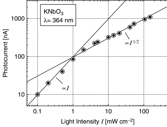
FIGURE 7.1. Photocurrent as a function of light intensity under interband illumination of KNbO 3 . In the low intensity regime, the photocurrent increases linearly and charge recombination in deep traps plays a major role. In the high intensity regime, the photocurrent increases with the square root of light intensity and interband transitions dominate the process. (After [13])
