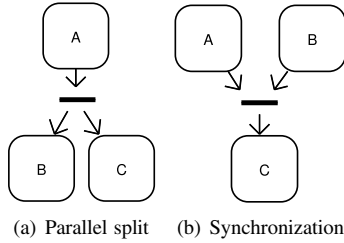
Figure 3. UML-S split and synchronization
