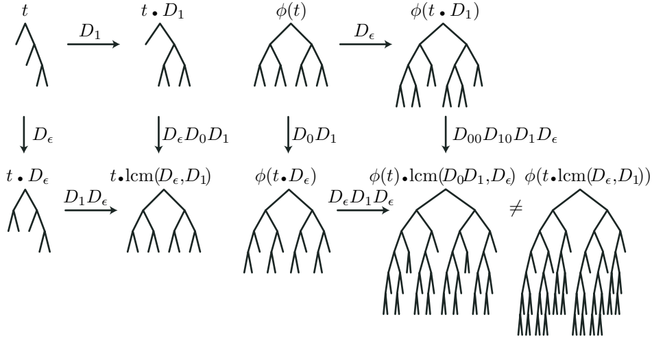
FIGURE 8. The left diagram shows an instance of Relation (6.4): for the considered choice of t , we find \Delta_t = D_\epsilon D_1 D_\epsilon , \Delta_{t \cdot D_1} = D_1 D_\epsilon D_0 D_{00} D_1 D_{10} , leading to \phi_t(D_1) = D_\epsilon and \phi_t(D_\epsilon) = D_0 D_1 . Here \phi_t(D_\epsilon) and \phi_t(D_1) are left-coprime, so (6.4) is true. The right diagram shows that the counterpart involving lcm's fails.
