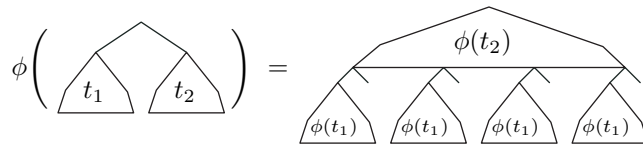
FIGURE 4. The fundamental LD-expansion \phi(t) of a term t , recursive definition: \phi(t_1 \star t_2) is obtained by distributing \phi(t_1) everywhere in \phi(t_2) .
