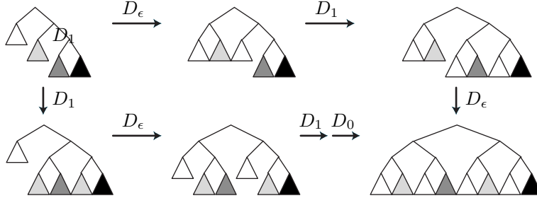
FIGURE 7. Relations between D_\alpha -expansions: the critical case. We read that the action of D_\epsilon D_1 D_\epsilon and D_1 D_\epsilon D_1 D_0 coincide.
