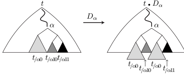
FIGURE 6. Action of D_\alpha to a term t : the LD-law is applied to expand t at position \alpha , i.e. , to replace the subterm t_{/\alpha} , which is t_{/\alpha 0} \star (t_{/\alpha 10} \star t_{/\alpha 11}) , with (t_{/\alpha 0} \star t_{/\alpha 10}) \star (t_{/\alpha 0} \star t_{/\alpha 11}) ; in other words, the light grey subtree is duplicated and distributed to the left of the dark grey and black subtrees.
