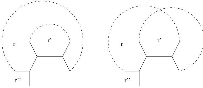
Figure 16: the proof that r_P(m_1) is quasi-regular.
