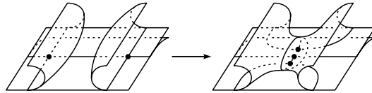
Figure 5: 2 \rightarrow 3 bumping move.
