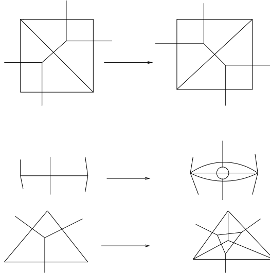
Figure 3: 2-dimensional moves
