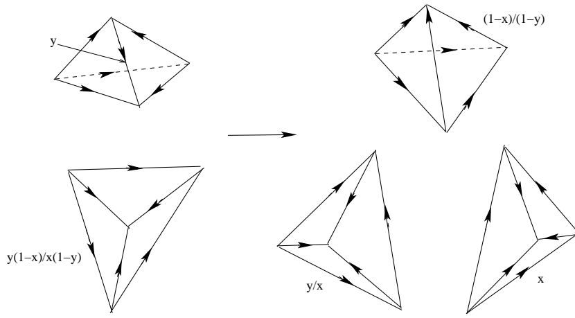
Figure 8: a 2 \leftrightarrow 3 ideal transit.
