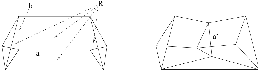
Figure 17: evolution of the geometric multiplicity of R when blowing-up a .
