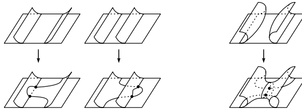
Figure 6: branched lune-moves.
