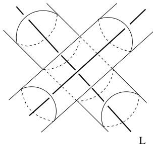
Figure 9: A tunnel junction over a diagram crossing.
