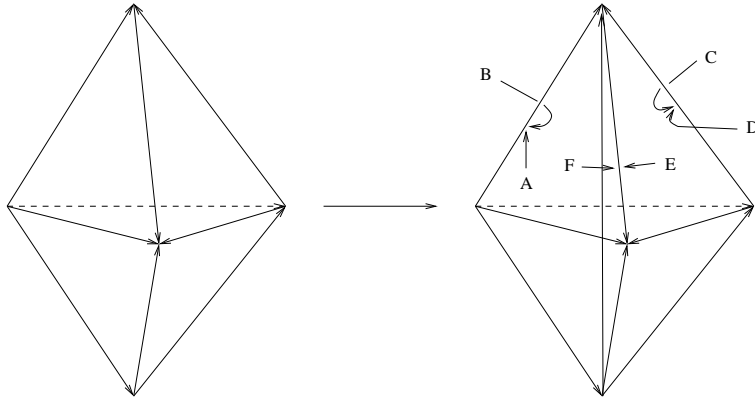
Figure 11: 2 \rightarrow 3 charge transits are generated by Neumann's vectors w(e) .
