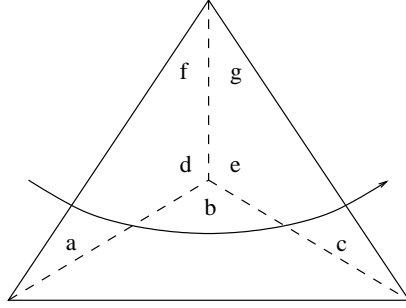
Figure 12: proof of 4.5 (2) for c_2 .
