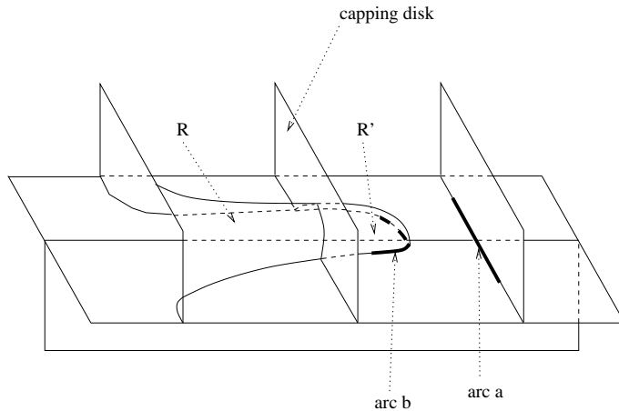
Figure 14: Capping disks are no obstructions for moves.
