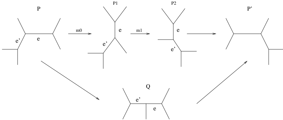
Figure 15: the 2-dimensional analogue of Prop. 4.23.
