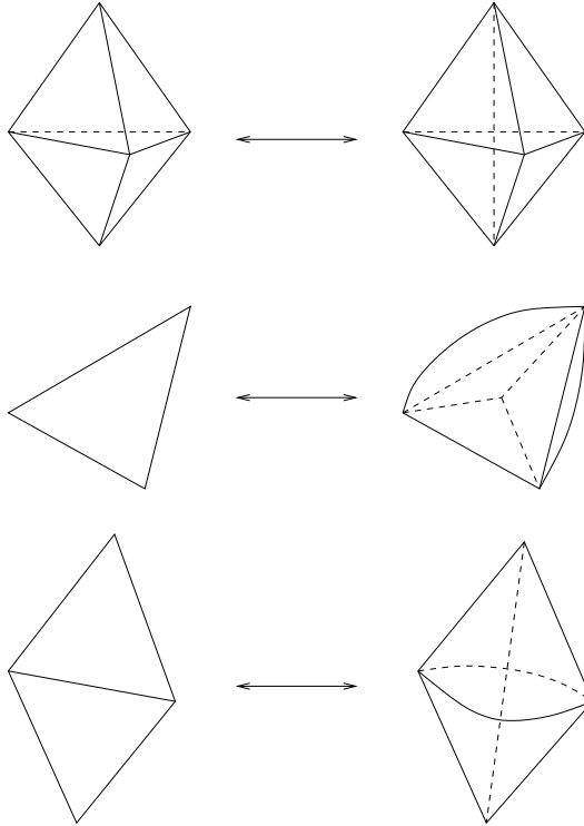
Figure 1: the moves between singular triangulations.
