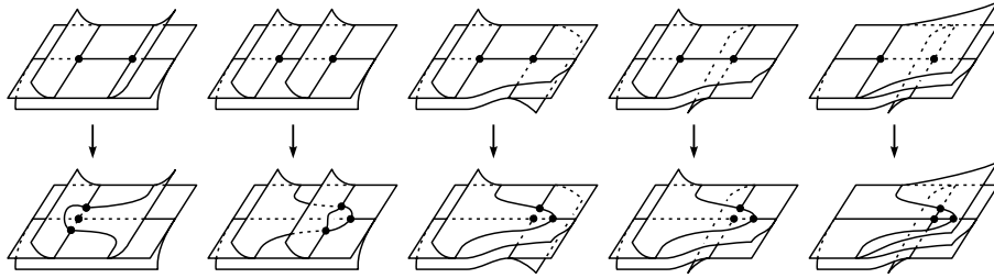
Figure 4: 2 \rightarrow 3 sliding moves.
