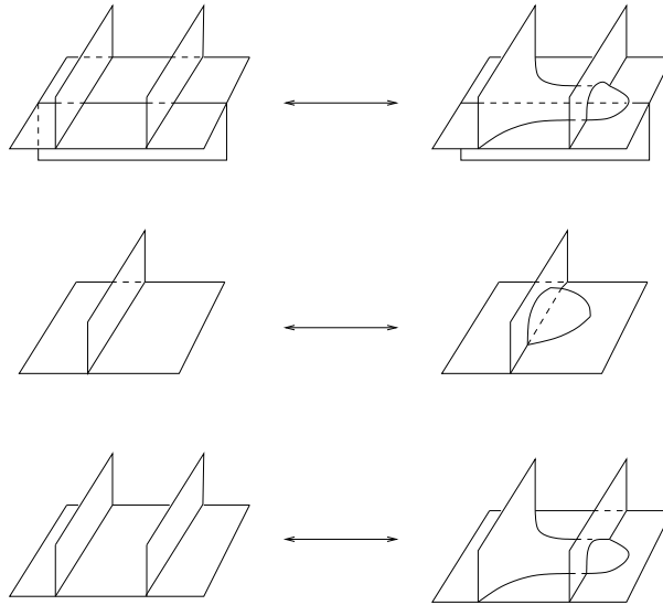
Figure 2: the moves on standard spines.
