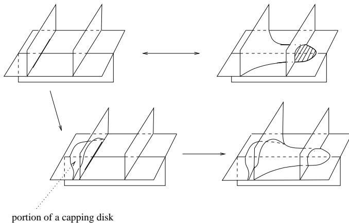
Figure 13: a non-quasi-regular move, and how to repair it by capping off the sector of immersion of the corresponding 3-cell.
