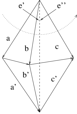
Figure 7: the compatibility relation around an edge.
