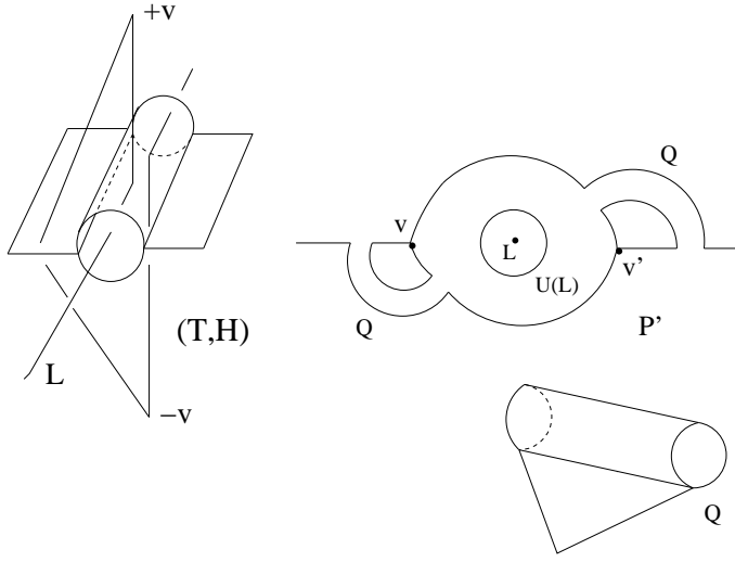
Figure 10: Final steps of the constructions of (T, H) and T' .
