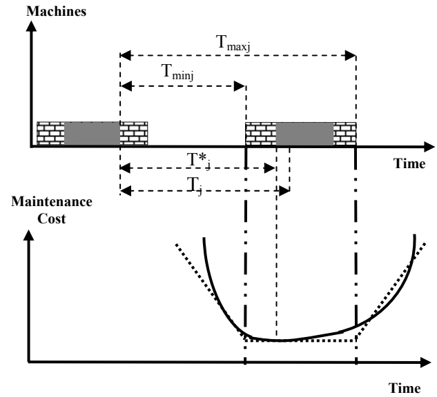
Fig. 2. Tolerance interval of a maintenance task.
