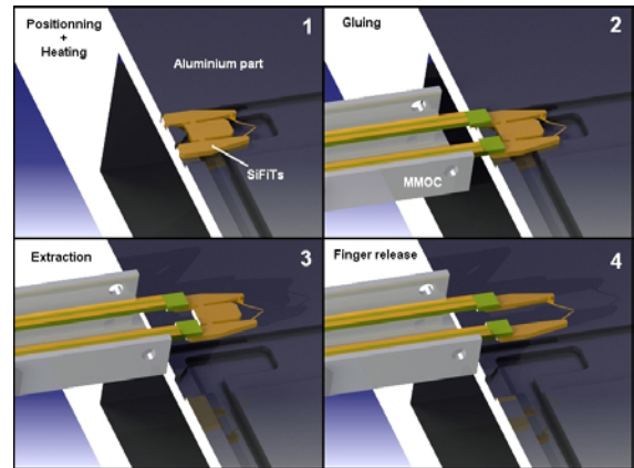
Fig. 6. Microgripper mounting process
