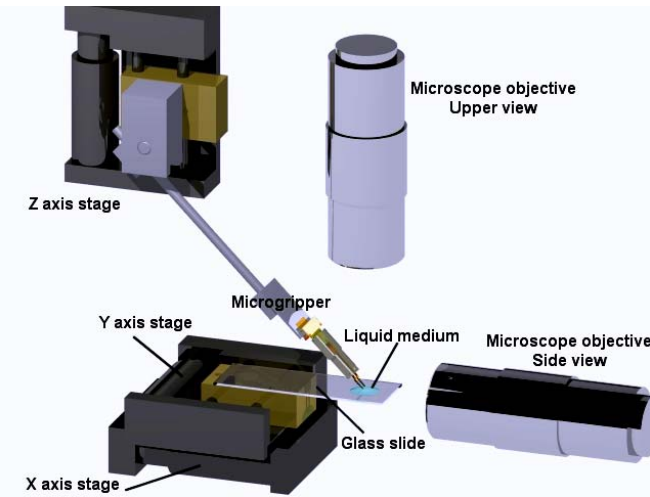
Fig. 2. Station setup
