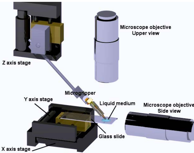
Fig. 2. Station setup
