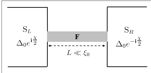
FIG. 1: SFS junction. The contact area are far smaller than the typical superconducting lead ( S_L, S_R ) transverse size. The metallic ferromagnet (F) in the middle part can be either two- or three- dimensional.
