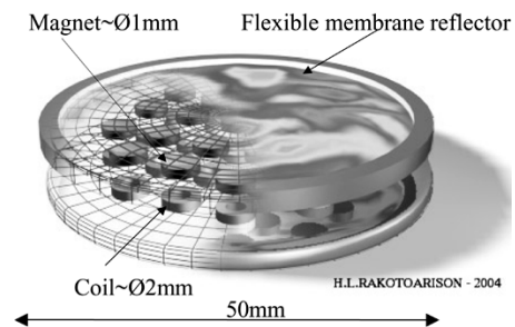
Fig. 4. Electromagnetic deformable mirror.
