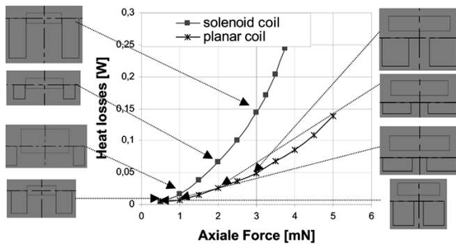
Fig. 10. Comparison showing the effectiveness of the planar coil.
