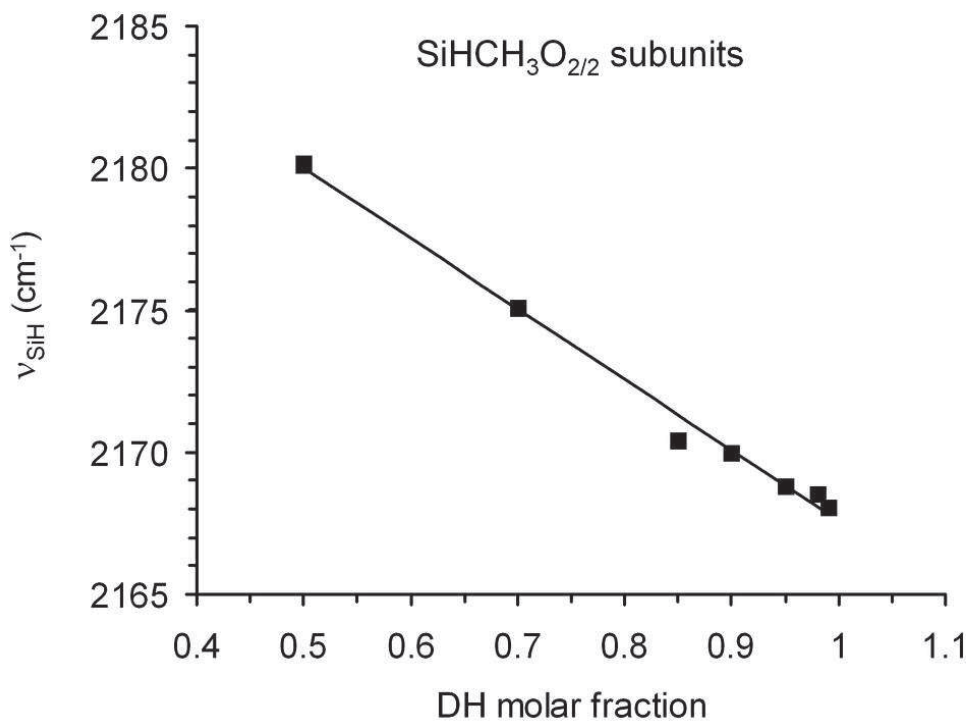
Figure 2. Si-H stretching peak position \nu_{\text{SiH}} of SiHCH 3 O 2/2 subunit as a function of the DH molar fraction in crosslinked PMHS thin films (ca. 1 \mu\text{m} ). The straight line corresponds to the least square fit of the experimental data: \nu_{\text{max}} (\text{cm}^{-1}) = -24.7 \alpha + 2192.7 where \alpha is the DH molar fraction.
