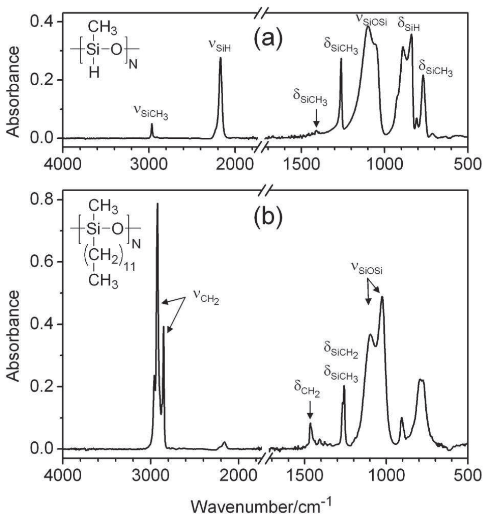
Figure 4. Transmission FTIR spectra of (a) virgin PMHS95 thin film (1.1 \mu m) and (b) after dodecyl functionalization via catalytic hydrosilylation (same sample).
