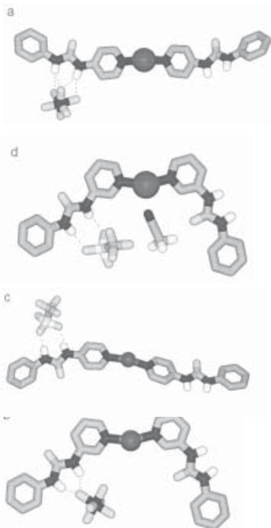
Fig. 1. Stick representation of the crystal structure of silver complexes a) [1_2\text{Ag}]^+\text{PF}_6^- 3 b) [2_2\text{Ag}]^+\text{PF}_6^- 4 , c) [1_2\text{Ag}]^+\text{CF}_3\text{SO}_3^- 5 and d) [2_2\text{Ag}]^+\text{PF}_6^- 6 crystalline complexes indicating a linear or an angular relative disposition of the ligands and the specific H-bonding of the \text{PF}_6^- and \text{CF}_3\text{SO}_3^- anions. The aromatic H atoms are omitted for clarity
