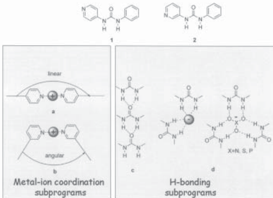
Scheme 1. Concept and design of molecular precursors 1 , 2 : a) linear and b) angular ion-coordination-directing structure scaffolds; c) urea head-to-tail and d) anion templating hydrogen-bonding supramolecular guiding subprograms
