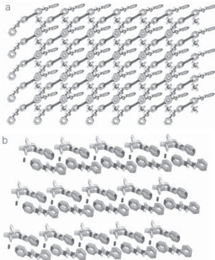
Fig. 3. a) Crystal packing of linear supramolecular rods of silver complexes a) [1/2\text{Ag}]^+\text{PF}_6^- ; 3 and b) [1/2\text{Ag}]^+\text{CF}_3\text{SO}_3^- ; 5 . The aromatic H atoms are omitted for clarity
