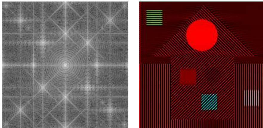
Fig. 2 \hat{I}_{Q_1, e_1 e_4} : Log-modulus (left) and directional cut filtering (right) for the red color
