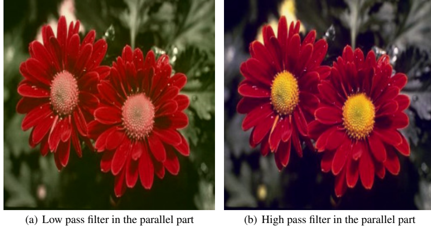
Fig. 4 The Clifford-Fourier transform \hat{F}_{Q_1, \frac{\nu\alpha \wedge e_4}{\|\nu\alpha \wedge e_4\|}} , with \alpha = (96, 109, 65)
