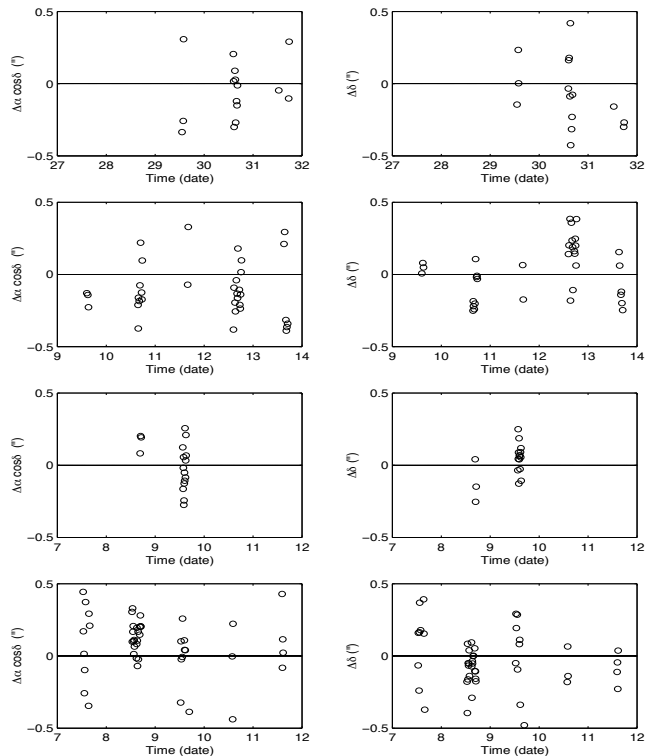
Figure 2. O-C of Nereid in 2006-2007 relative to the four sets of observations 216a, 216b, 100a and 100b from above to below
