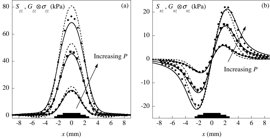
Fig. 3. Validation of the calibration procedure. Measured stress profiles under normal loading by the rigid cylinder ( P=0.69 N ( \bullet ), 1.72 N ( \blacksquare ) and 2.75 N ( \blacklozenge ) (a) normal stress S_{zz}(x) and (b) tangential stress S_{xz}(x) . Comparison is made with G_{zz} \otimes \sigma_{zz}(x) and G_{xz} \otimes \sigma_{xz}(x) for \mu_s=0 (solid lines) and \mu_s = \infty (dashed lines). The black rectangular patches on the x axis represent the contact widths (3.00, 4.50 and 5.34 mm for P=0.69 , 1.72 and 2.75 N, respectively) obtained from the finite elements calculations for \mu_s=0 .
