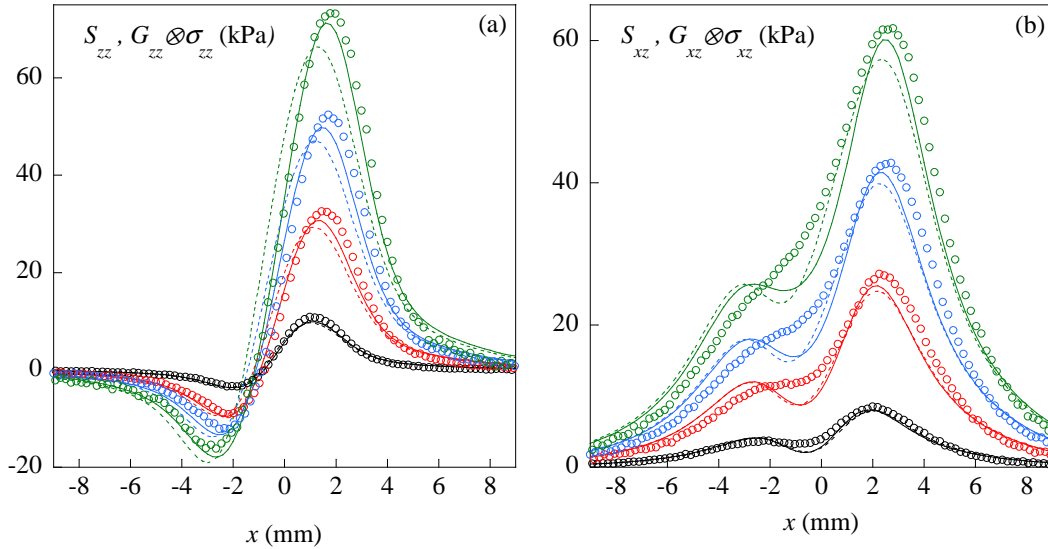
Fig. 10. Measured stress profiles (o, for clarity only one percent of the data points is shown) at y=0 (a) S_{zz} and (b) S_{xz} in steady sliding regime for increasing normal loads ( P=0.34 N in black, 1.03 N in red, 1.72 N in blue and 2.75 N in green) and V=1 mm.s^{-1} . Comparison is made with (a) G_{zz} \otimes \sigma_{zz} and (b) G_{xz} \otimes \sigma_{xz} where \sigma_{zz} and \sigma_{xz} are computed from the exact model (solid lines) or from Goodman's model (dashed lines).
