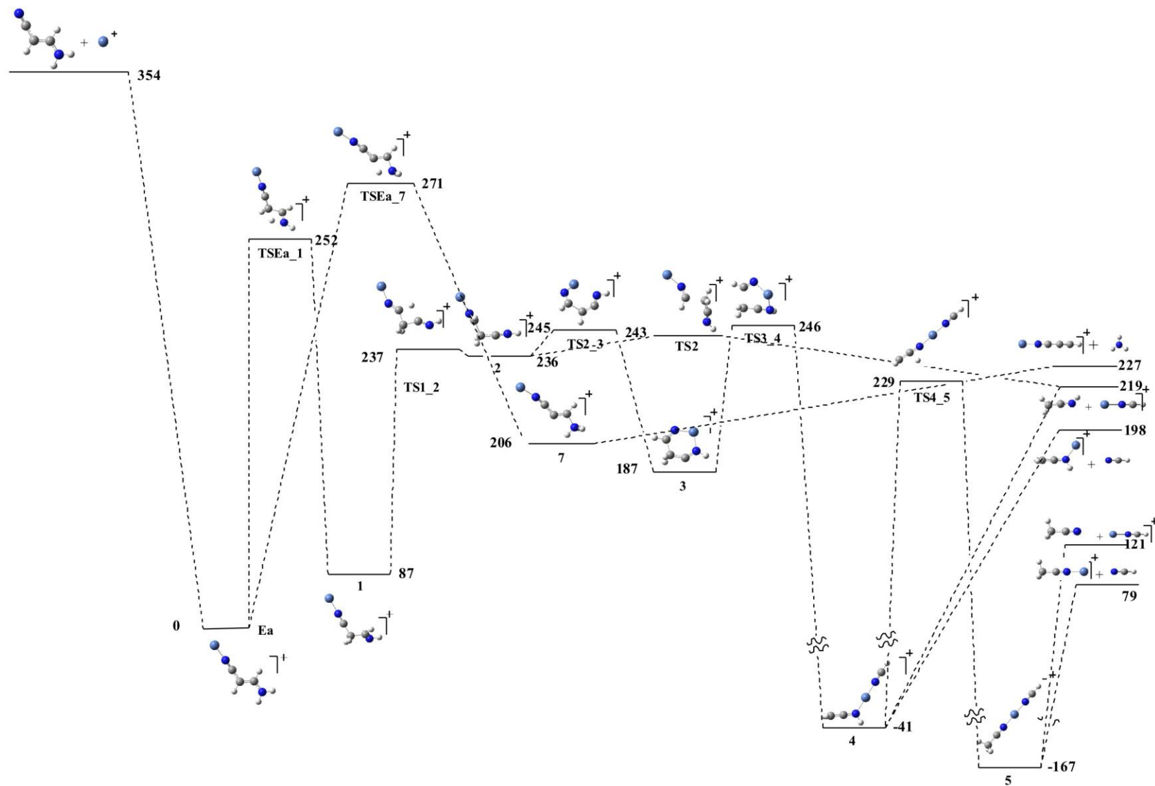
Figure 3. Energy profile of the mechanisms associated with the loss of HCN, C 2 N, H 3 and NH 3 . Relative energies in kJ/mol
