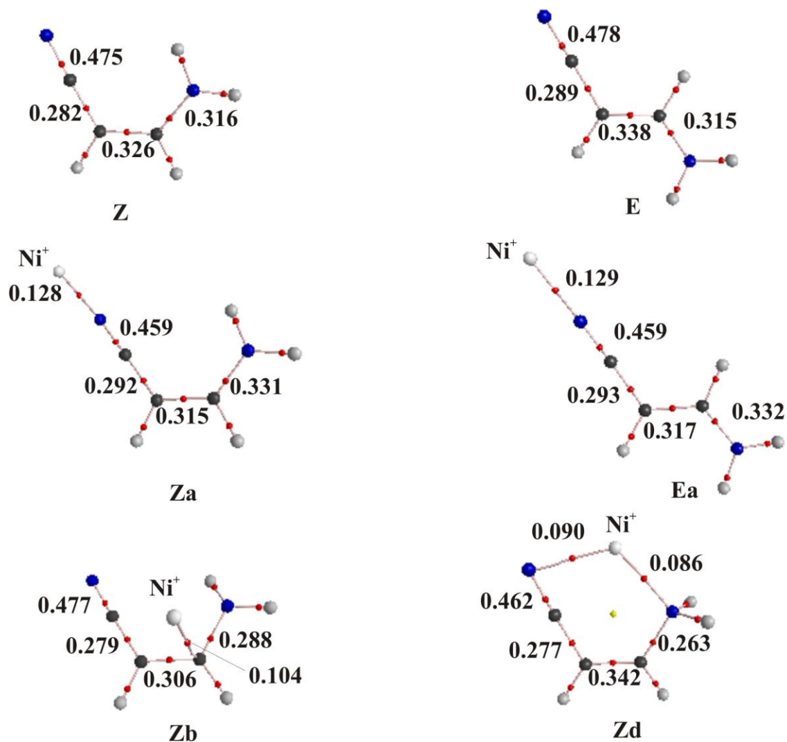
Figure 2. Molecular graphs, showing the bond critical points and the bond paths of the two isomers, E and Z, of aminoacrylonitrile and their most stable Ni + adducts. Electron densities are in a.u.
