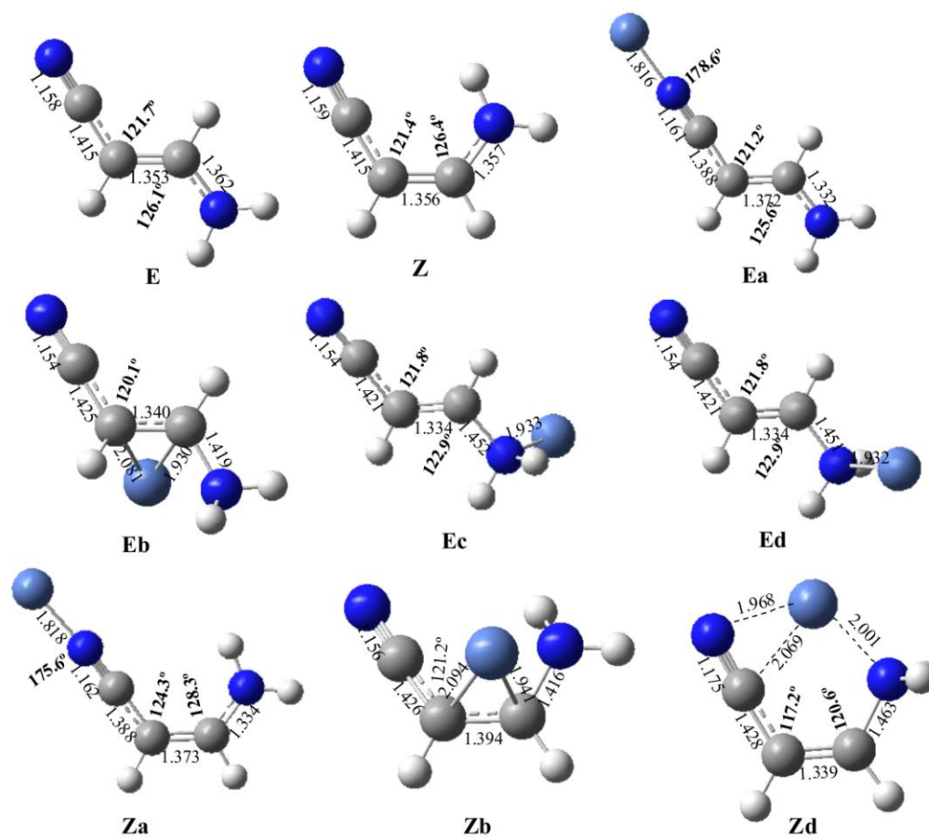
Figure 1. B3LYP/6-311G(d,p) optimized geometries of the two isomers, E and Z, of aminoacrylonitrile and their \text{Ni}^+ adducts. Bond lengths are in Å and bond angles in degrees.
