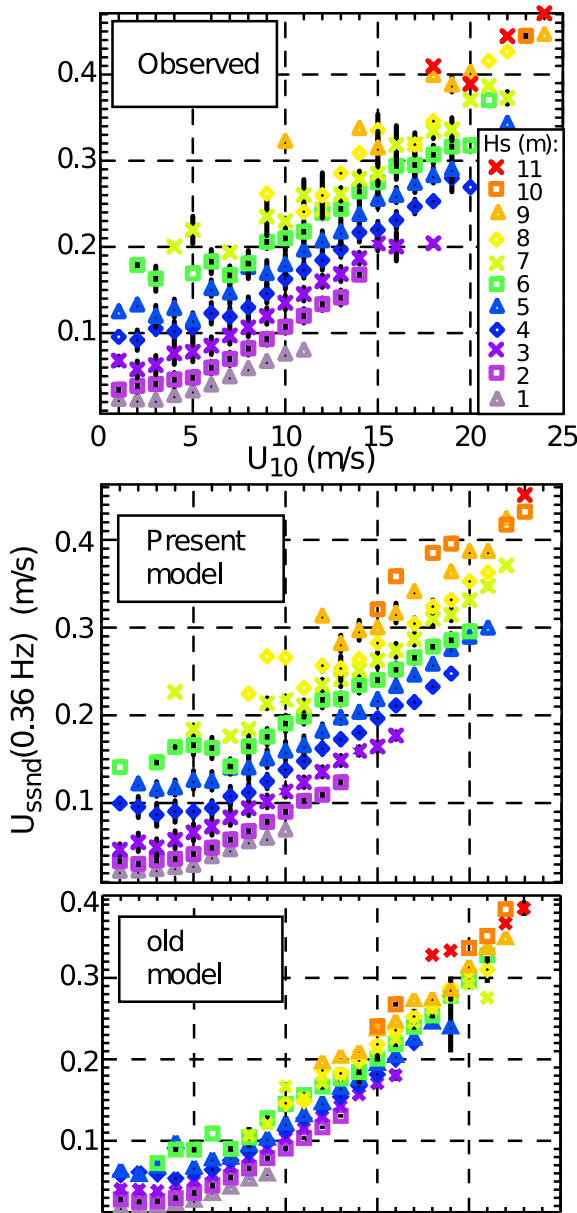
FIG. C1. Variation of the wave spectrum third moment, m_3 converted to a velocity U_{\text{ssnd}} = (2\pi)^3 m_3(f_c)/g , that would equal the surface Stokes drift in deep water if all waves propagated in the same direction. For each data source a cut-off frequency of f_c = f_B = 0.36 Hz is taken and the data is binned wind speed, at 1 \text{ m s}^{-1} intervals, and significant wave height H_s (in colors) at 1 \text{ m} intervals from 1 to 11 \text{ m} . The top panel shows buoy data offshore of Oregon (NDBC buoy 46005), the middle panel shows present model results, and the bottom panel shows results from the same model but using the parameterization of Bidlot et al. (2007), including a factor F = 2.5 . The vertical error bars indicate plus and minus half the standard deviation of the data values in each (U_{10}, H_s) class.
