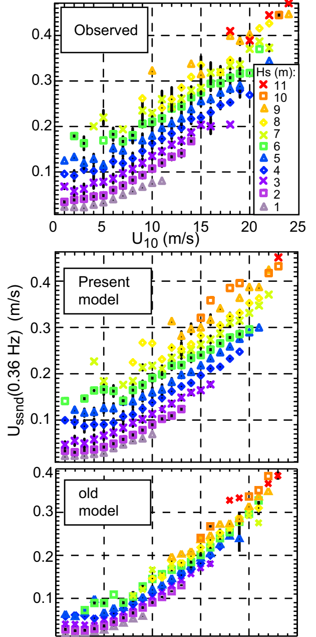
FIG. C1. Variation of the wave spectrum third moment, m_3 converted to a velocity U_{ssnd} = (2\pi)^3 m_3(f_c)/g , that would equal the surface Stokes drift in deep water if all waves propagated in the same direction. For each data source a cut-off frequency of f_c = f_B = 0.36 Hz is taken and the data is binned wind speed, at 1 \text{ m s}^{-1} intervals, and significant wave height H_s (in colors) at 1 m intervals from 1 to 11 m. The top panel shows buoy data offshore of Oregon (NDBC buoy 46005), the middle panel shows present model results, and the bottom panel shows results from the same model but using the parameterization of Bidlot et al. (2005), including a factor F = 2.5 . The vertical error bars indicate plus and minus half the standard deviation of the data values in each (U_{10}, H_s) class.
