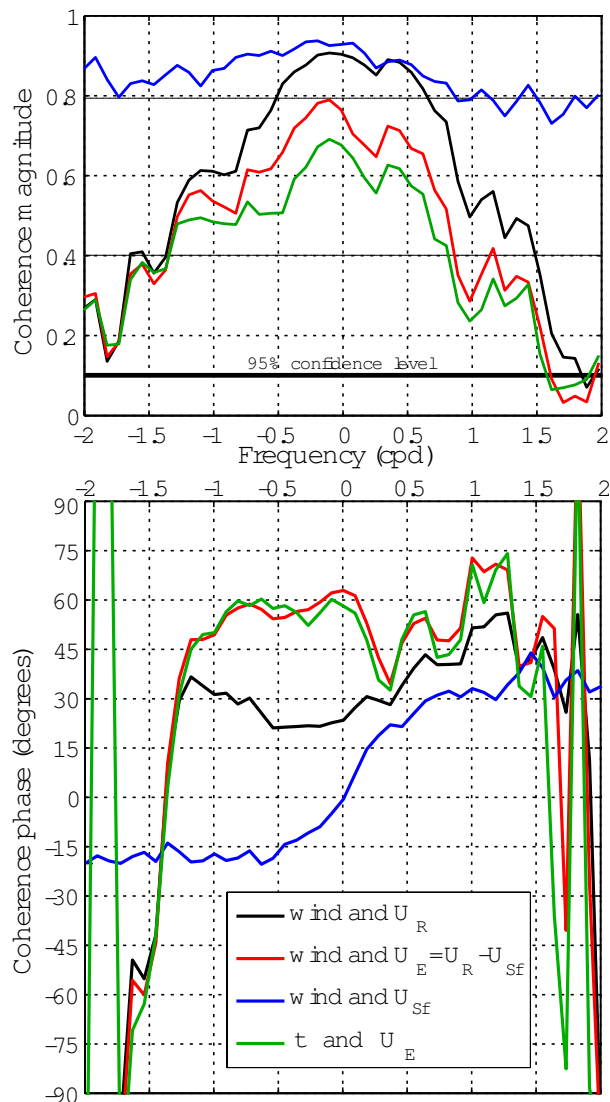
FIG. 4. Rotary co-spectra of the wind and wind stress with the radar-derived current, Stokes drift and Eulerian current. (a) magnitude and (b) phase. The number of degrees of freedom is 108 at the spectral resolution of 0.09 cpd. Coherence is significant at the 95% confidence level for a value of 0.1. Negative and positive frequencies are clockwise and counter-clockwise polarized motions, respectively.
