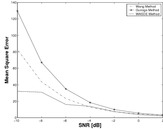
Figure 4. Mean square error for various SNR
