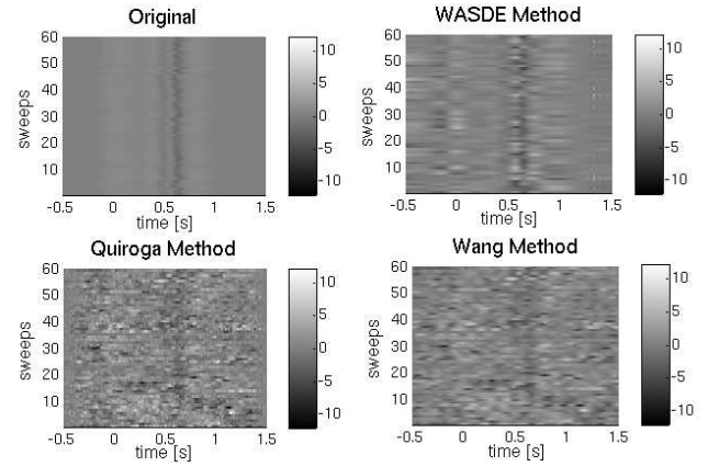
Figure 3. Comparison of three methods (Wasde, Guiroga and Wang), for a SNR = -10dB
