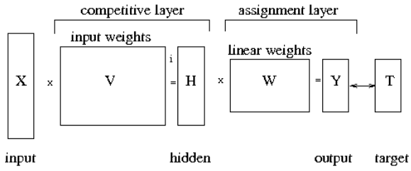
Figure 1. Generic architecture for LVQ algorithms
