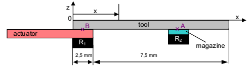
Fig. 4. Sketch of the system used in the modeling process.
