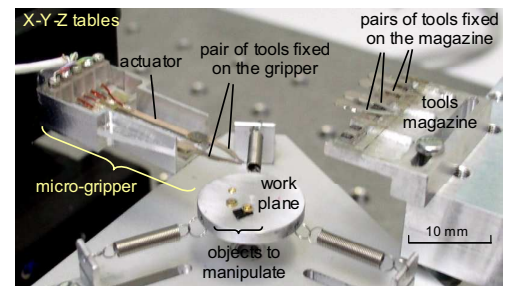
Fig. 1. Different parts of the micromanipulation station: a microgripper composed of a piezo-actuator and a pair of tools is fixed on micro-positioning tables. The objects to manipulate are placed on a work plane and several pairs of tools are available in a tools magazine.
