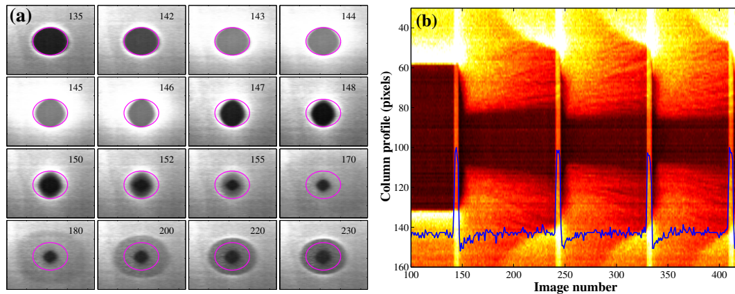
Figure 1: Simultaneous record of dust cloud and central plasma glow during the heartbeat instability: (a) direct images, (b) time evolution of central column profile (in false colors), the superimposed curve is the plasma glow in the void central pixel.
