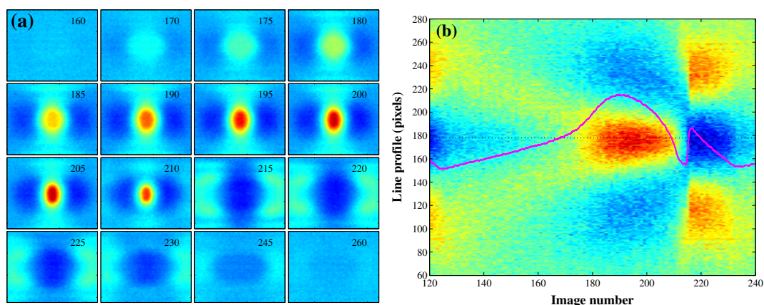
Figure 2: Plasma glow in the whole volume, (a) post-processed images in false colors, (b) time evolution of central line profile with electrical measurements superimposed.
