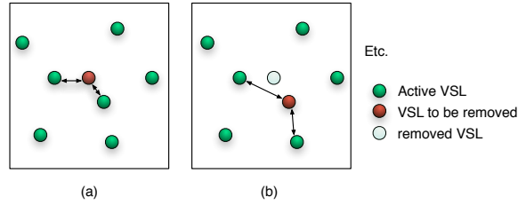
Figure 5: Removing additional VSLs is performed choosing the VSL having the closest distance to its 2 closest neighbors: (a) first VSL removal; (b) removing a second VSL requires updating all the distances d_{min1} and d_{min2} .
