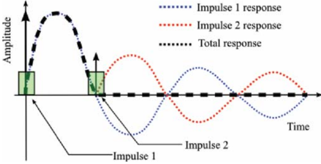
Figure 5. Basic idea of Input Shaping for two impulse response.
