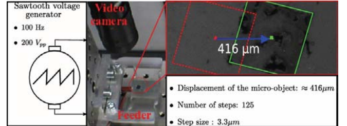
Figure 11. Vibrating experiment.
