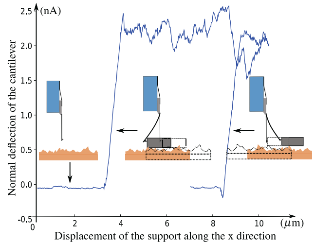
Figure 9. Example of force curve
