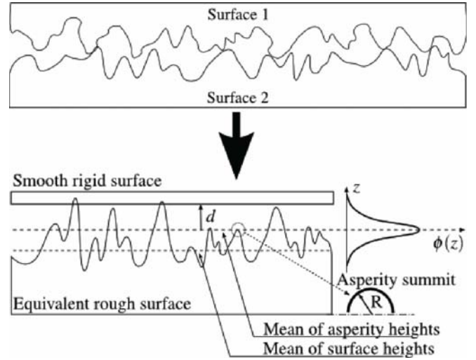
Figure 8. Greenwood-Williamson model of contact mechanics
