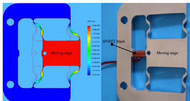
Figure 1. Feeder using inertial force: Feeder by inertial force. (Left) Simulation of the displacement of the table along the X direction, (Right) photograph of the feeder and his high voltage piezoelectric actuator.
