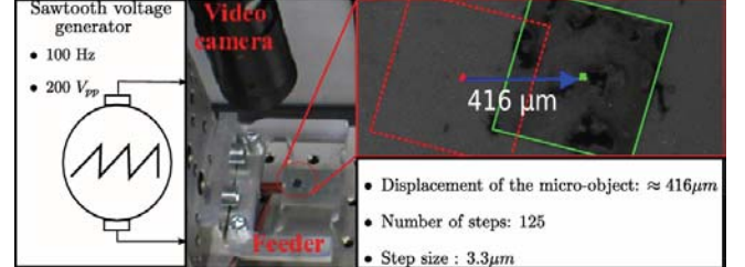
Figure 11. Vibrating experiment.
