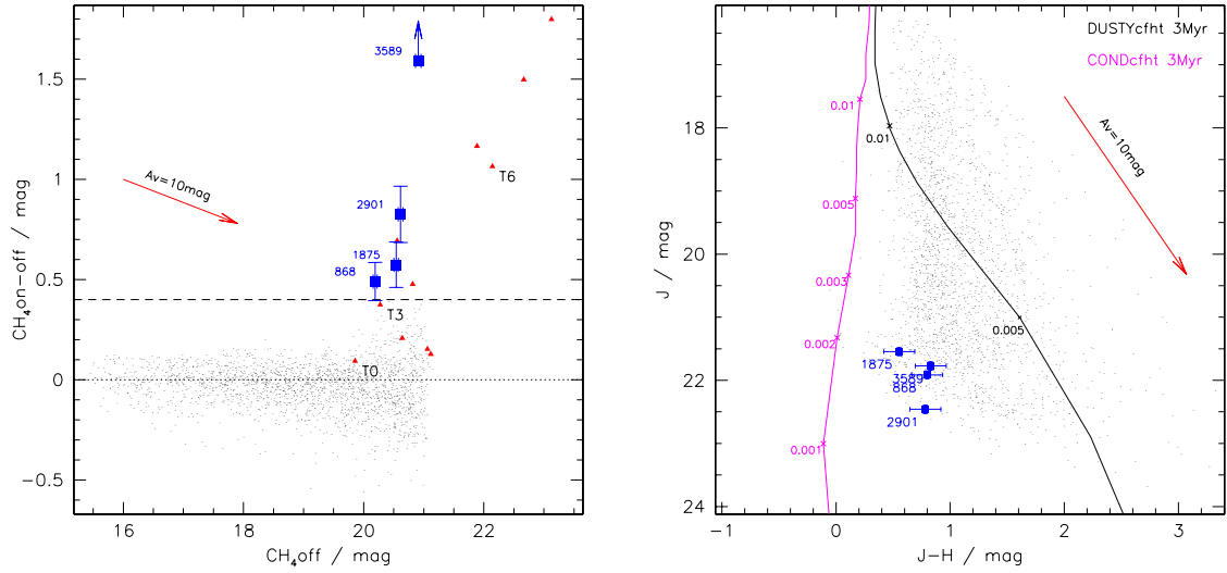
FIGURE 2. Left : Observed CH_{4on}-CH_{4off} colours versus CH_{4off} magnitude for stars in our survey. The 4 candidate T-dwarfs are shown as blue squares. The field T0-T7 dwarf sequence, shifted to a distance of 340 pc, is shown for reference (red triangles). At an age of 3 Myr, IC 348 T-dwarfs are expected to be brighter than field dwarfs, as are the 4 identified candidates. An extinction vector of A_V=10 \text{ mag} is shown. Note the asymmetric distribution of the CH_{4on}-CH_{4off} colours in this diagram, with more field objects with negative values, due to extinction. Right : J versus (J-H) colour-magnitude diagram. Dusty (black) and Cond (magenta) 3 Myr isochrones are shown as solid lines labelled with mass ( M_{\odot} ). An A_V=10 \text{ mag} extinction vector is shown. IC 348 T-dwarf candidates are shown as blue squares. They lie between Dusty and Cond isochrones as expected for intermediate T-dwarfs.
