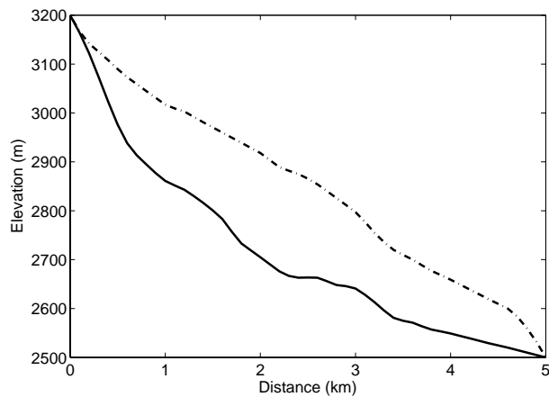
Fig. 4. Surface and bedrock profile of Haut Glacier d'Arolla.
