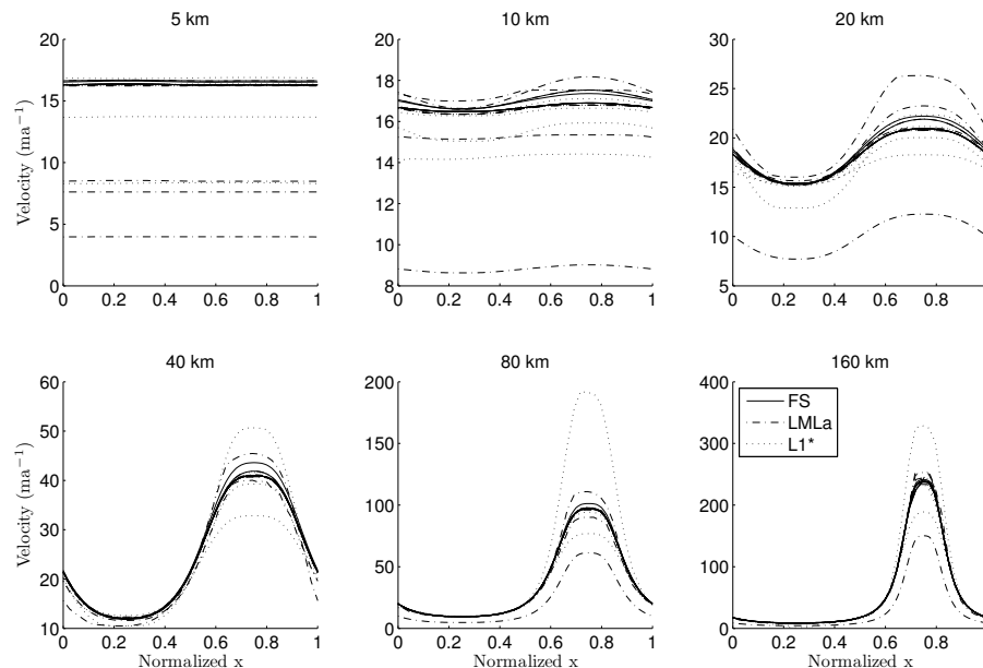
Fig. 10. Results for Exp. C. Surface velocity across the bump at y=L/4 for different length scales L .
