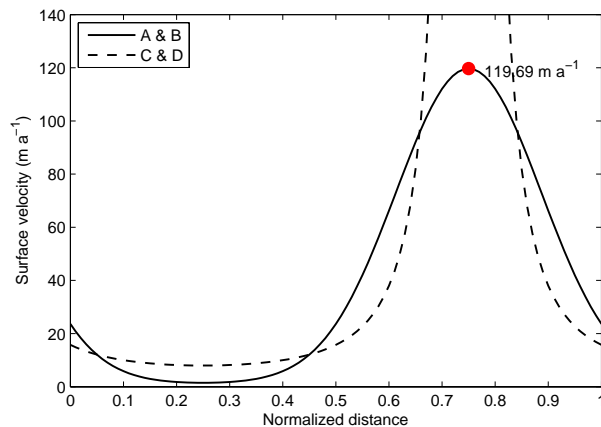
Fig. 8. Surface velocity profiles along y=L/4 according to the analytical SIA solution for Exps. A–D, based on Eqs. (28) and (29). Results are independent of L .
