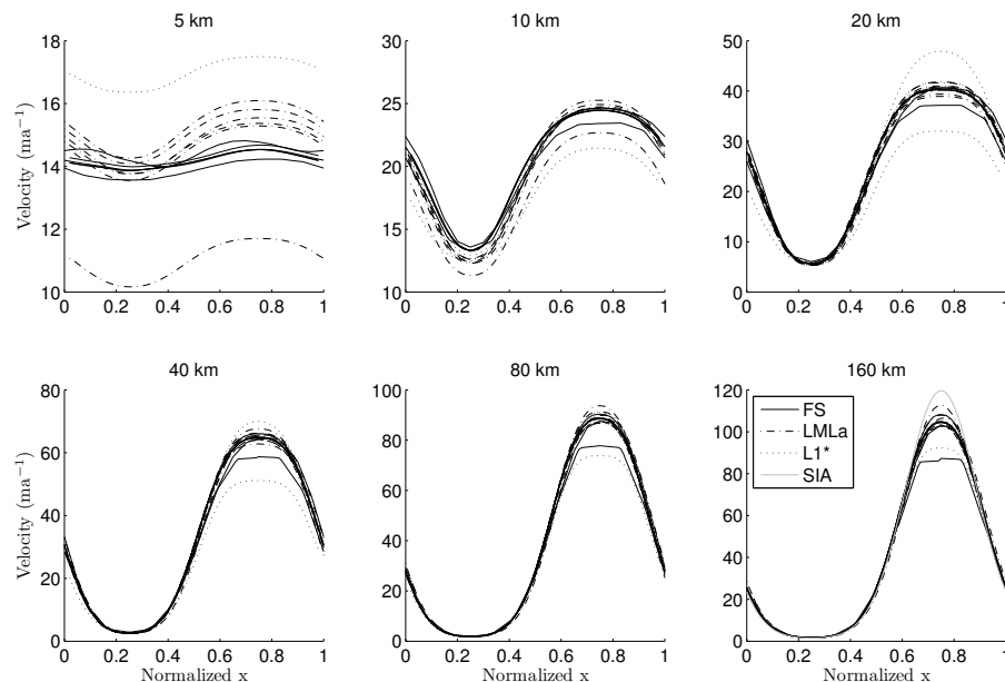
Fig. 6. Results for Exp. A. Surface velocity across the bump at y=L/4 for different length scales L .
