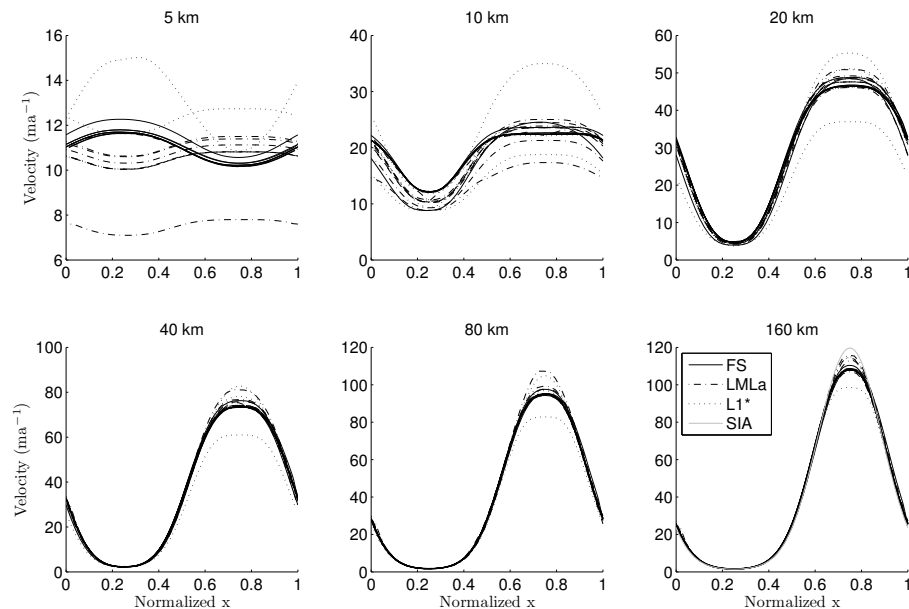
Fig. 7. Results for Exp. B. Surface velocity for different length scales L .
