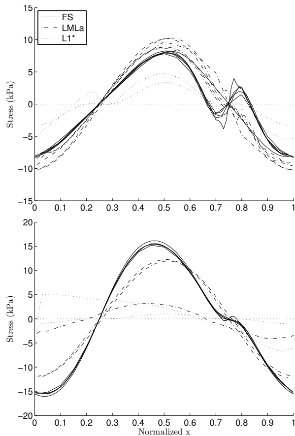
Fig. 12. Basal pressure difference according to Exp. C for L=10 and 5 km, respectively.
