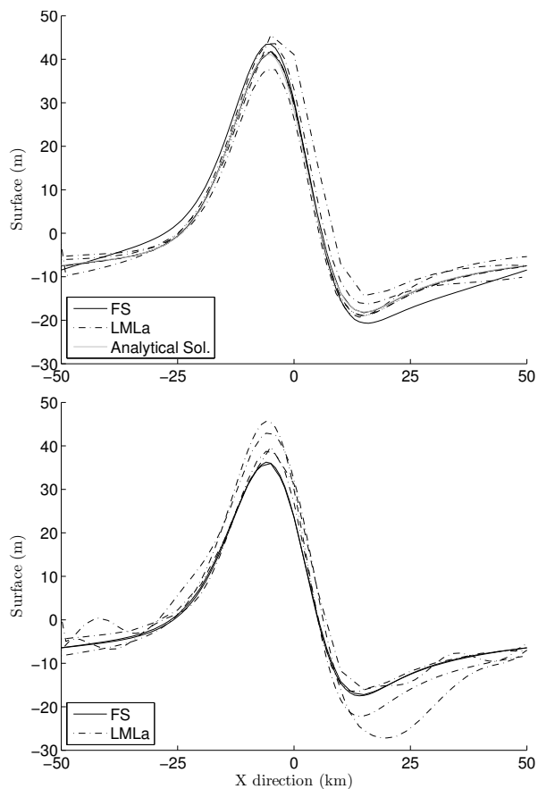
Fig. 15. Steady state surface elevation along the central flowline for Exp. F for the no sliding (top) and sliding (bottom) experiment.
