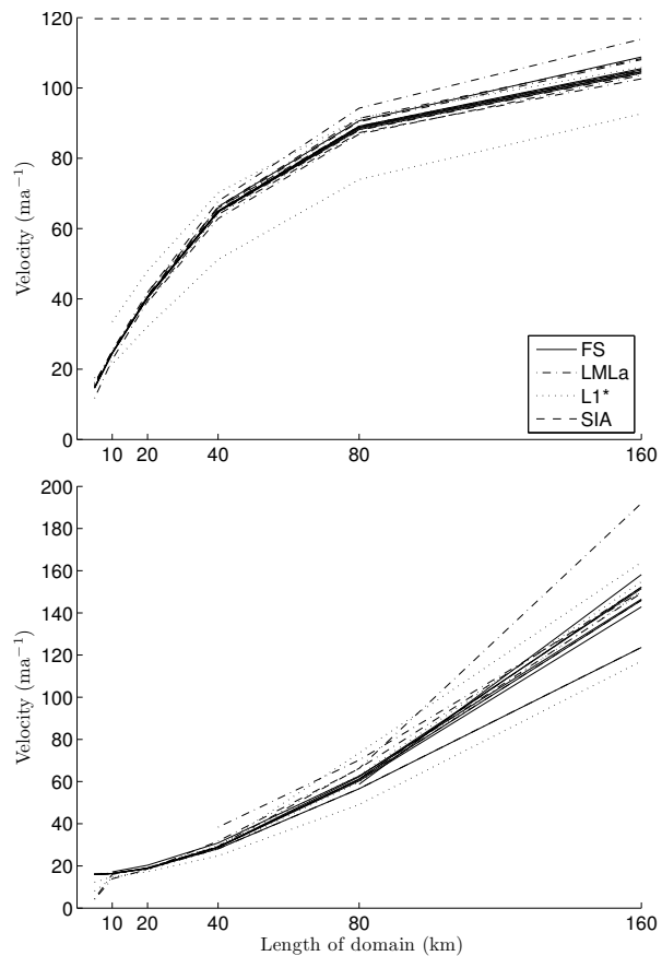
Fig. 11. Results for Exp. D. Surface velocity for different length scales L .
