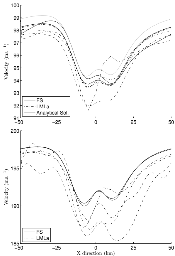
Fig. 16. Steady state surface velocity along the central flowline for Exp. F for the no sliding (top) and sliding (bottom) experiment.
