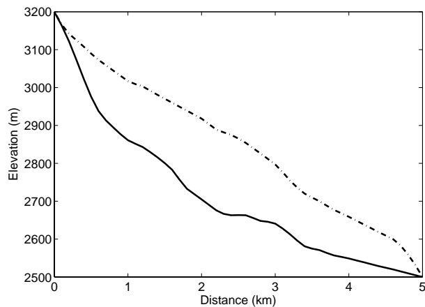
Fig. 4. Surface and bedrock profile of Haut Glacier d'Arolla.
