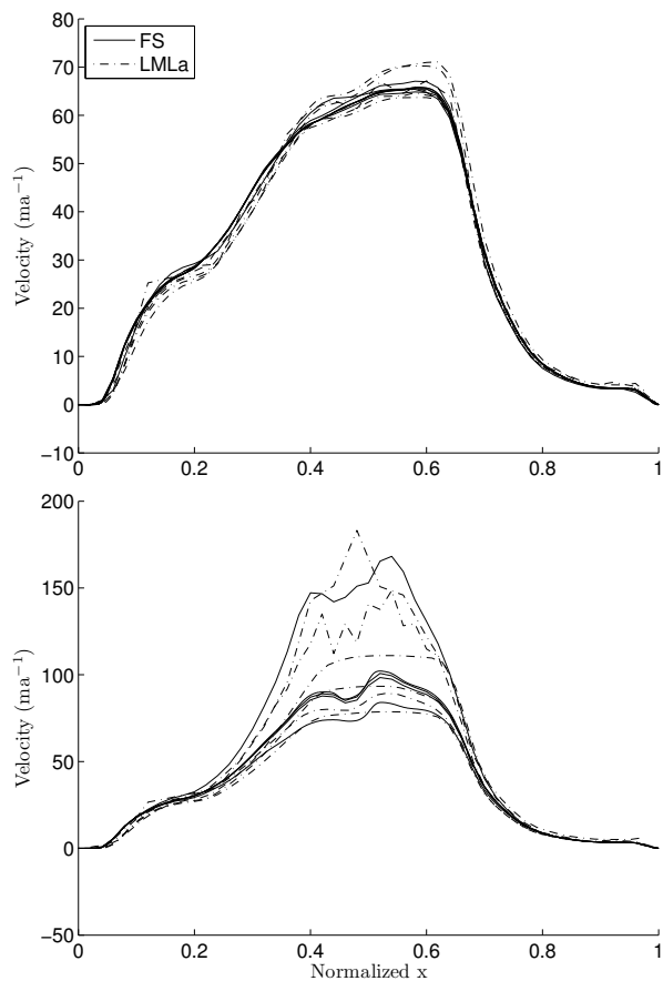
Fig. 13. Surface velocity in the direction of the ice flow for Exp. E for the no-sliding (top) and sliding (bottom) experiment.
