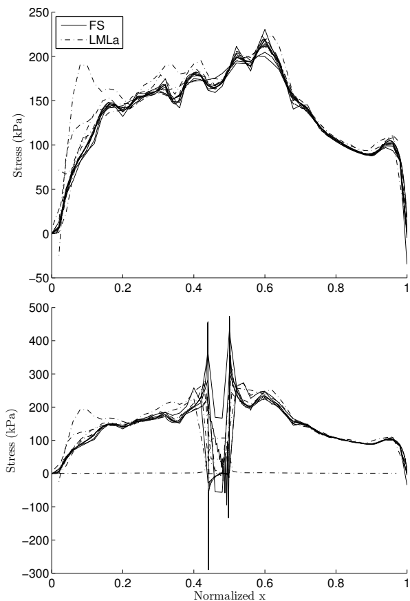
Fig. 14. Basal shear stress in the direction of the ice flow for Exp. E for the no-sliding (top) and sliding (bottom) experiment.
