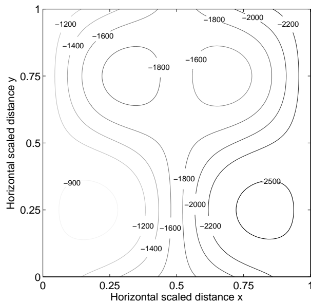
Fig. 2. Basal topography z_b (m) for Exp. A according to Eq. (14) for L=80 km. Ice flow is from left to right.
