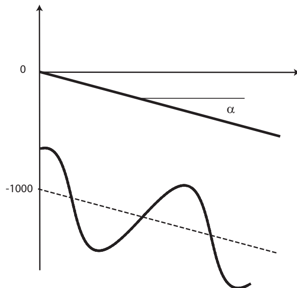
Fig. 1. Cartesian coordinate system used for Exp. A–D.
