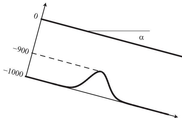
Fig. 5. Tilted coordinate system used for Exp. F.
