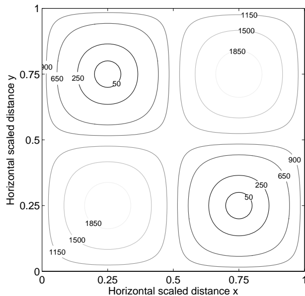
Fig. 3. Basal friction coefficient \beta^2 for Exp. C.
