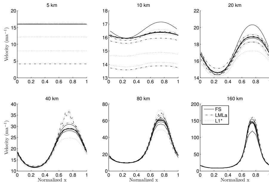
Fig. 9. Maximum surface velocity in the direction of the ice flow for Exp. A (top) and C (bottom) as a function of length scale L . Graphs for Exps. B and D are similar.
