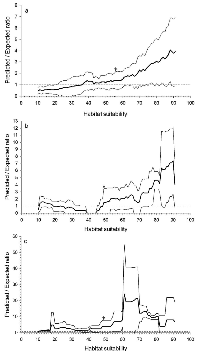
Fig. 2. Predicted-to-expected ratio curve (mean \pm SD) and threshold between unsuitable and suitable areas (arrow) for (a) sperm whale, (b) pilot whale and (c) Risso's dolphin models (the limit of random models, predicted-to-expected ratio F_i=1 , is indicated by the dotted line).
