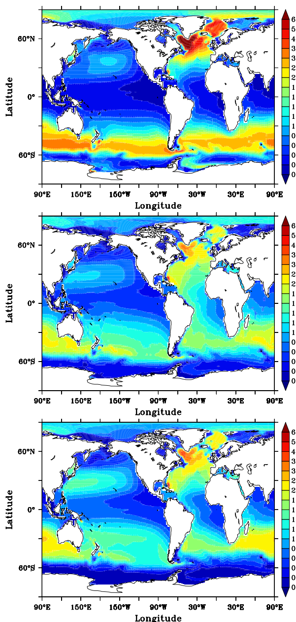
Fig. 14. Normalised inventories simulated in the noneddying model obtained by dividing by the mean area-weighted inventory for CFC-11 (top), anthropogenic CO 2 (middle), and bomb \Delta^{14}\text{C} (bottom) at end of year 1994.
