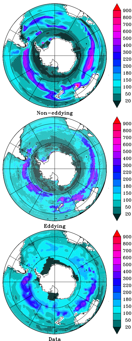
Fig. 4. Mixed-layer depth (m) in the southern extratropics in mid-September as simulated by the noneddy (top) and eddy (middle) models as well as that from an observational climatology (de Boyer Montégut et al., 2004) (bottom).
