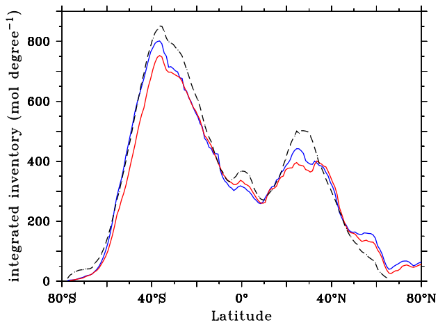
Fig. 9. Global zonal integral of the bomb \Delta^{14}\text{C} inventory as observed (black dashes, GLODAP) and as simulated by the noneddying (blue) and eddying (red) models at end of year 1994.
