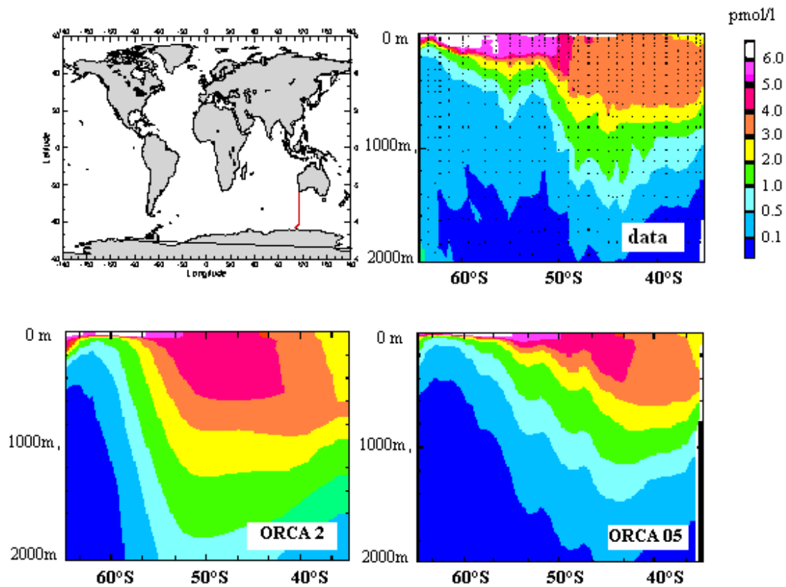
Fig. 6. CFC-11 concentration (in \text{pmol l}^{-1} ) along the WOCE I9S section ( 115^\circ \text{ E} , 1994–1995) as observed and simulated by the noneddying (ORCA2) and the eddying (ORCA05) model.
