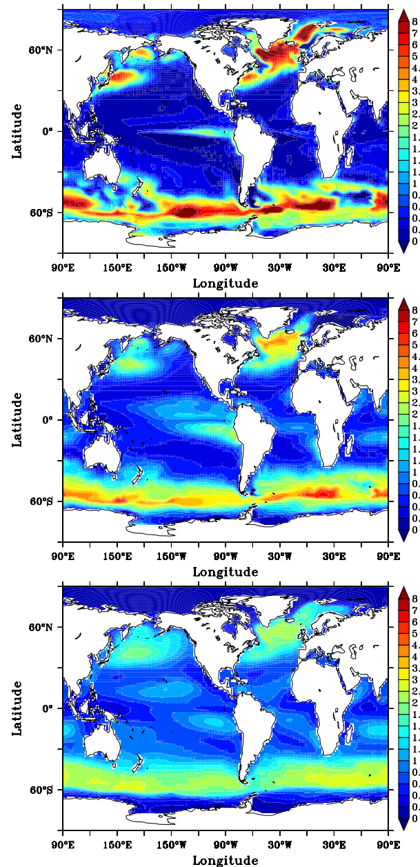
Fig. 12. Normalised cumulative fluxes simulated by the noneddying model for CFC-11 (upper), anthropogenic CO 2 (middle), and bomb \Delta^{14}\text{C} (lower), accumulated since the beginning of each simulation until the end of year 1994. Fluxes were normalised by dividing each field by the global area-weighted mean flux; thus there are no units.
