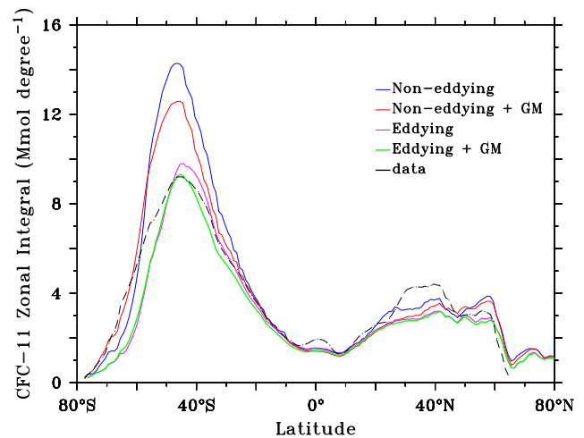
Fig. 2. Zonally integrated inventories of CFC-11 in 1994 as observed (black dashes, GLODAP) and as simulated by the noneddyling model with GM (red) and without GM (blue) as well as by the eddyling model with GM (green) and without GM (purple).
