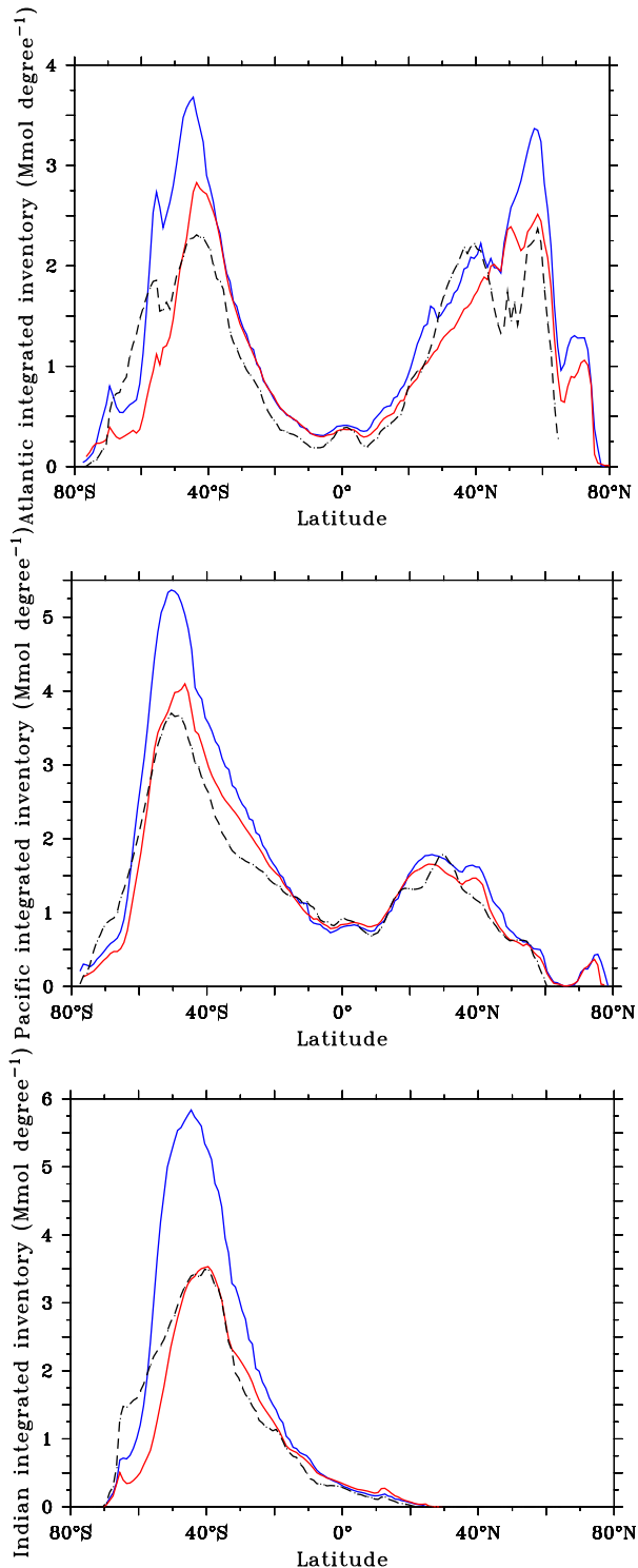
Fig. 3. Zonally integrated basin-scale inventories of CFC-11 for the Atlantic (upper), Pacific (middle), and Indian (lower) Oceans as observed (black dashes, GLODAP) and as simulated by the eddying (red) and noneddying (blue) models at end of year 1994.
