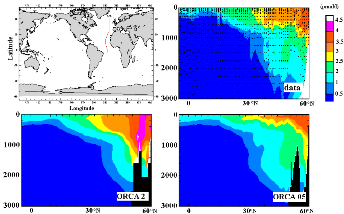
Fig. 8. CFC-11 concentration (in \text{pmol l}^{-1} ) along the Na20w section (1993) as observed and simulated by the noneddy (ORCA2) and the eddy (ORCA05) models
